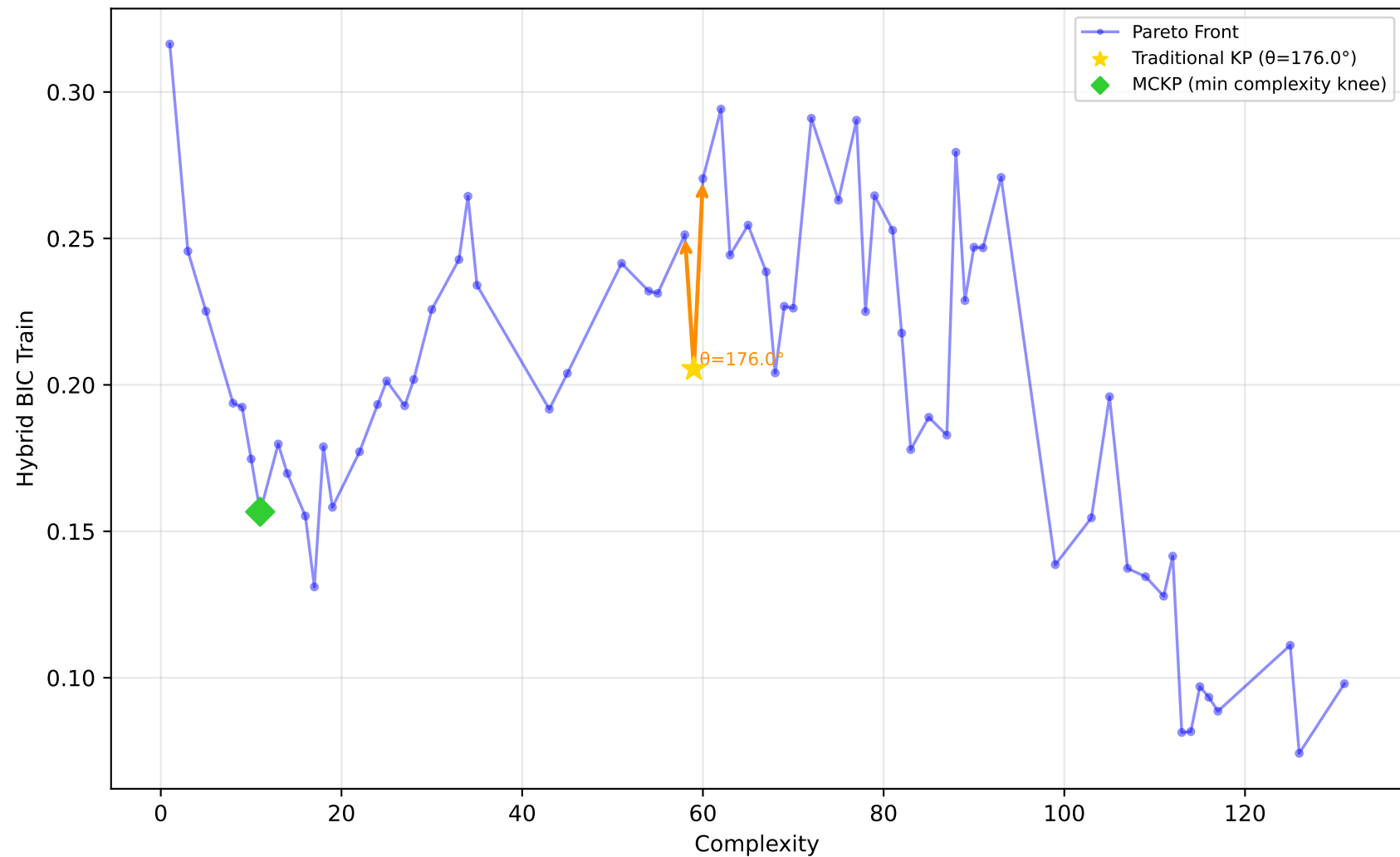
678_visualizing_environmental - Run 15 - SVP - Hybrid BIC Train \lambda_1=0.40, \lambda_2=0.00, \lambda_3=0.00 | Difficulty: 0.19 | Method: mckp
