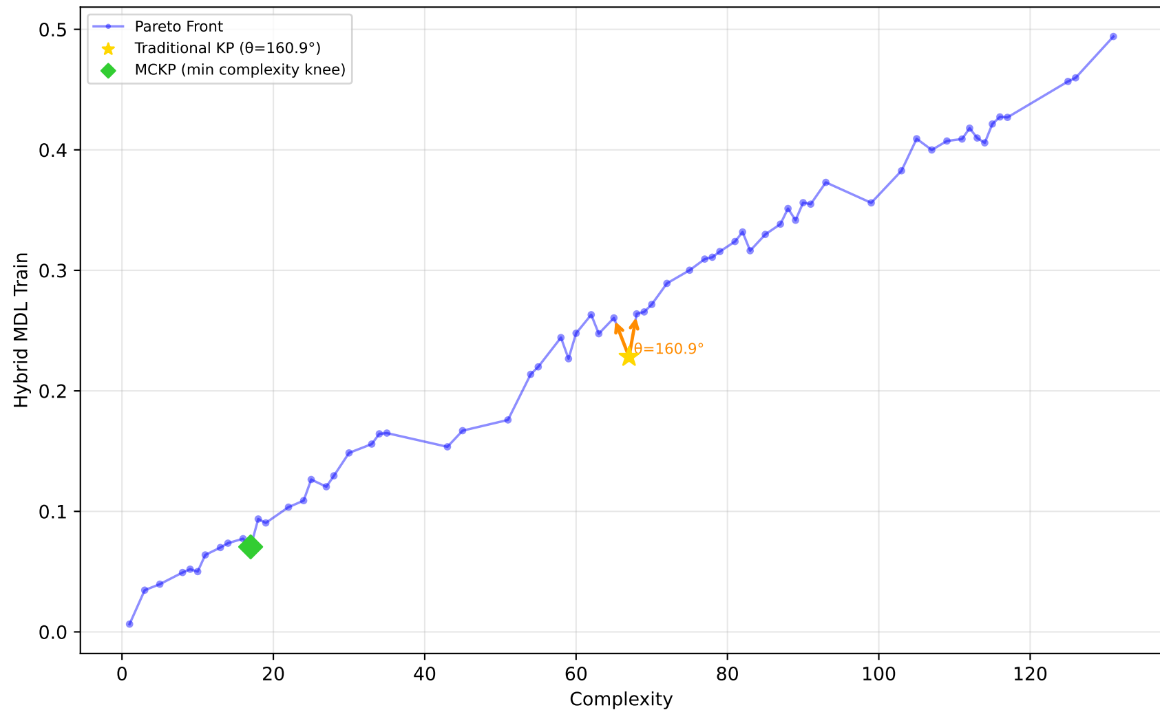
678_visualizing_environmental - Run 15 - SVP - Hybrid MDL Train \lambda_1=0.40, \lambda_2=0.00, \lambda_3=0.00 | Difficulty: 0.19 | Method: mckp
