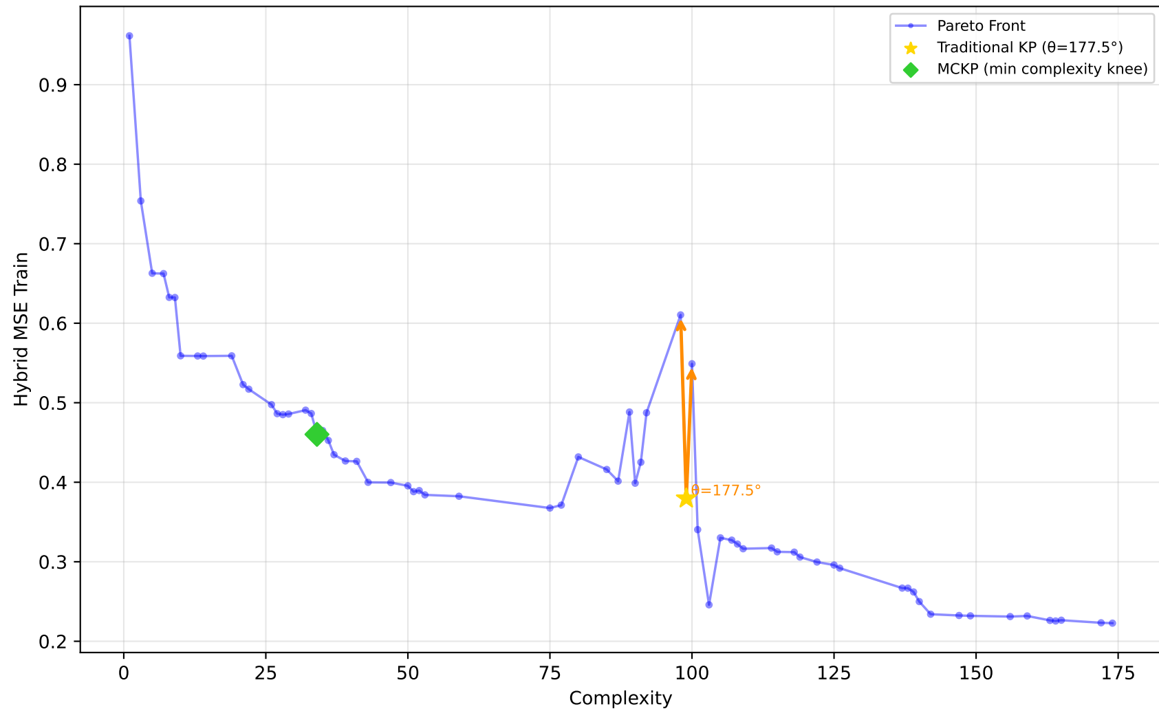
678_visualizing_environmental - Run 16 - MVP - Hybrid MSE Train \lambda_1=0.40, \lambda_2=0.00, \lambda_3=0.00 | Difficulty: 0.35 | Method: mckp
