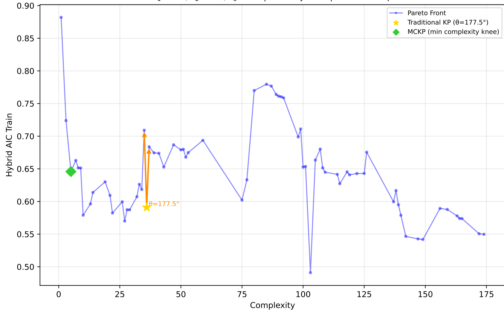
678_visualizing_environmental - Run 16 - SVP - Hybrid AIC Train \lambda_1=0.00, \lambda_2=0.10, \lambda_3=0.20 | Difficulty: 0.35 | Method: mckp
