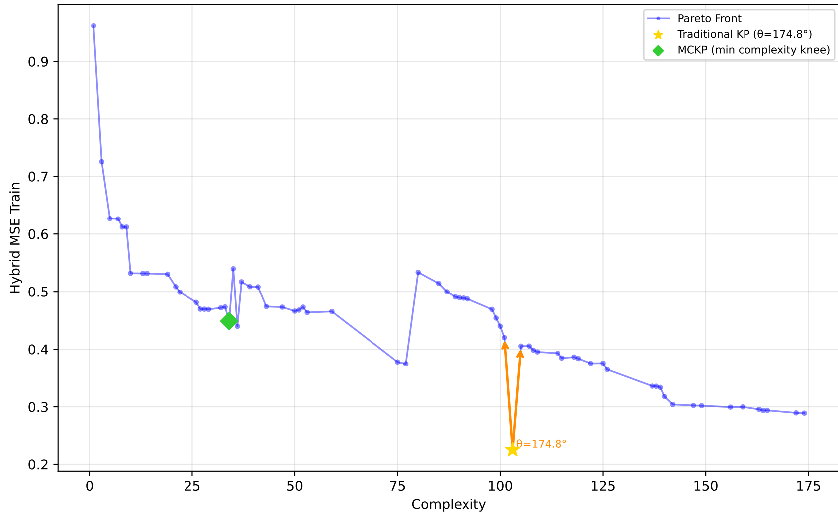
678_visualizing_environmental - Run 16 - SVP - Hybrid MSE Train \lambda_1=0.00, \lambda_2=0.10, \lambda_3=0.20 | Difficulty: 0.35 | Method: mckp
