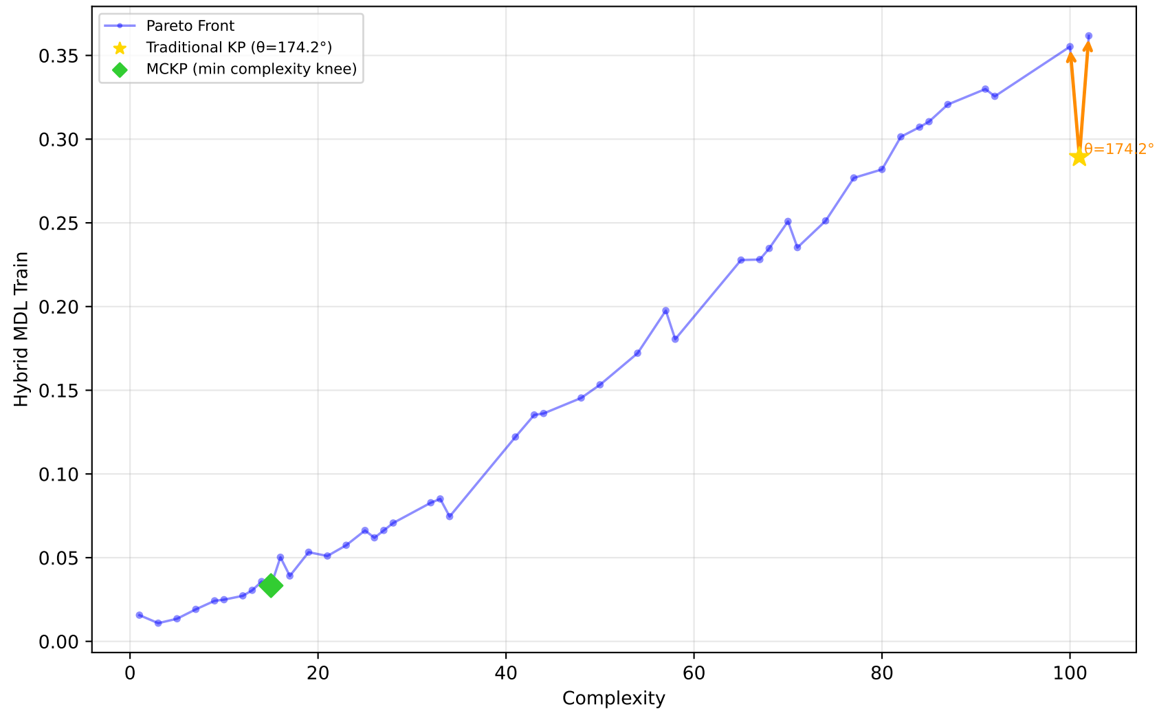
678_visualizing_environmental - Run 17 - MVP - Hybrid MDL Train \lambda_1=0.00, \lambda_2=0.00, \lambda_3=0.10 | Difficulty: 0.26 | Method: mckp
