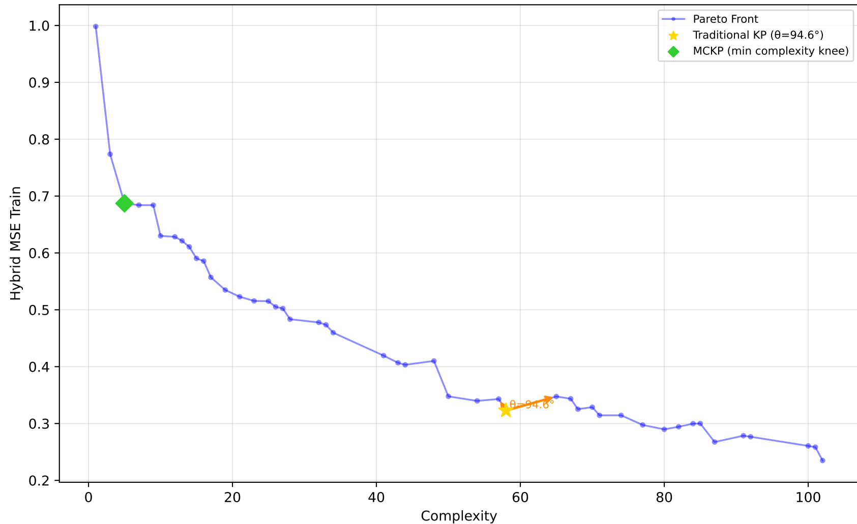
678_visualizing_environmental - Run 17 - MVP - Hybrid MSE Train \lambda_1=0.00, \lambda_2=0.00, \lambda_3=0.10 | Difficulty: 0.26 | Method: mckp
