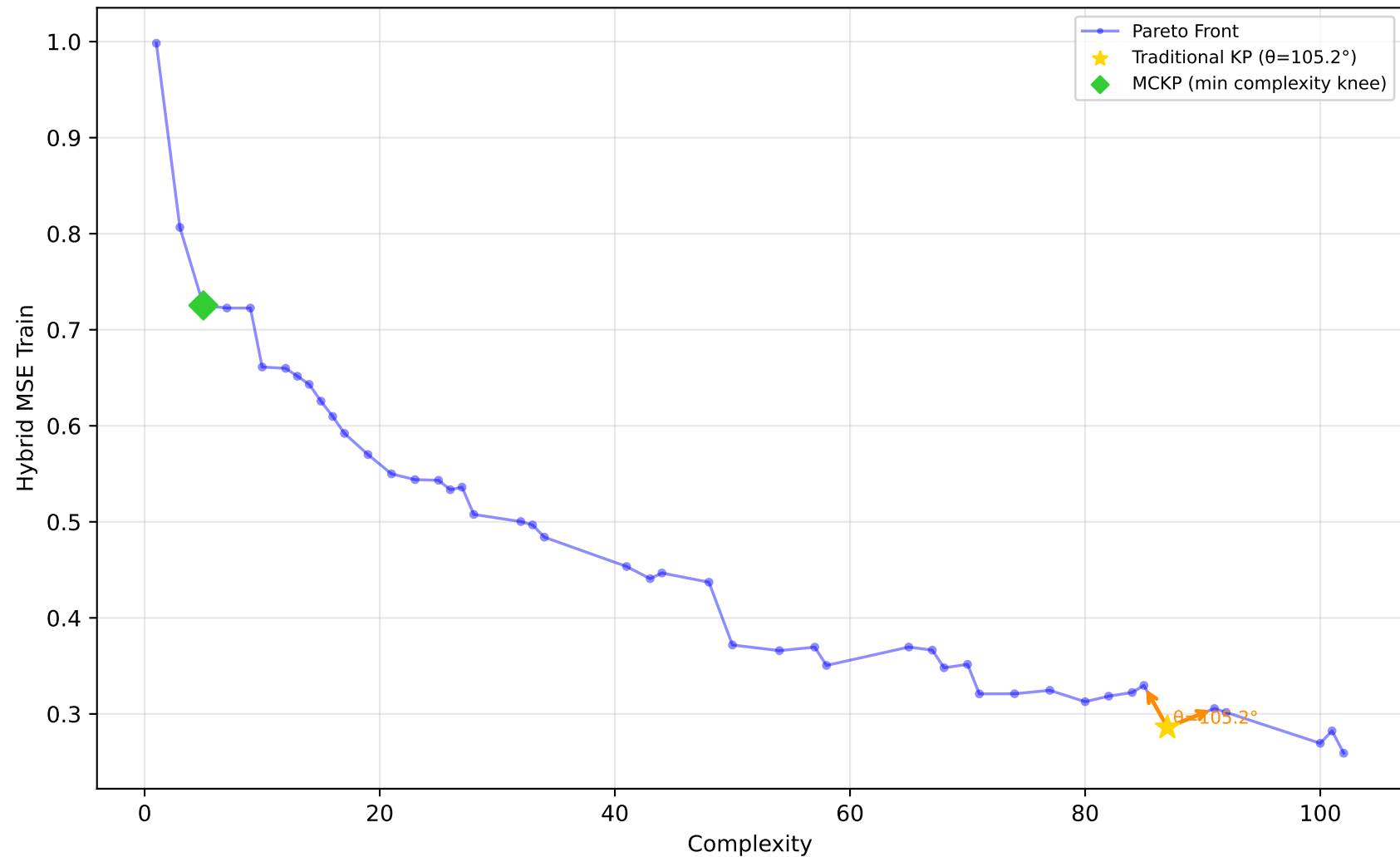
678_visualizing_environmental - Run 17 - MVP - Hybrid MSE Train \lambda_1=0.40, \lambda_2=0.00, \lambda_3=0.00 | Difficulty: 0.26 | Method: mckp
