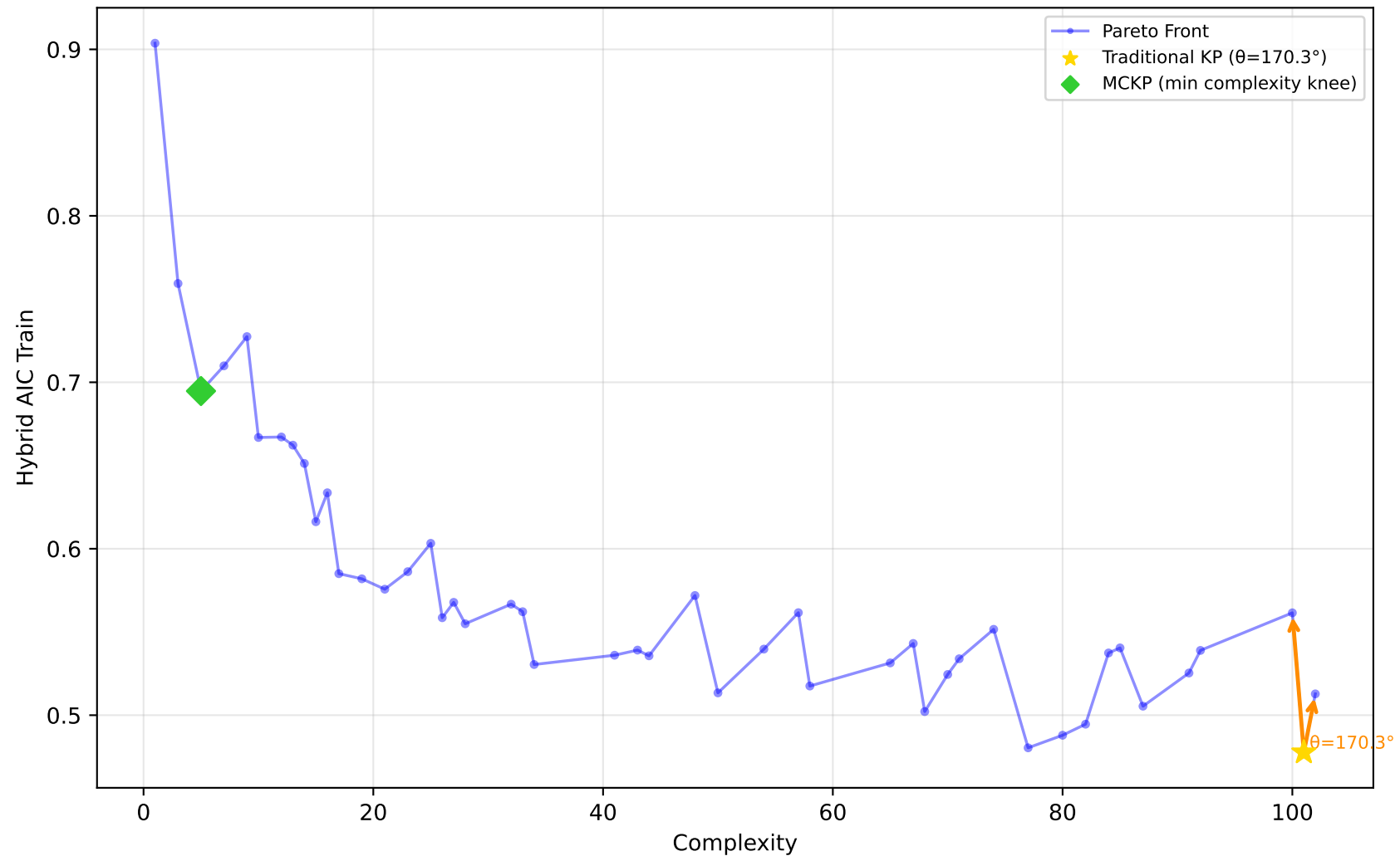
678_visualizing_environmental - Run 17 - SVP - Hybrid AIC Train \lambda_1=0.00 , \lambda_2=0.10 , \lambda_3=0.20 | Difficulty: 0.26 | Method: mckp
