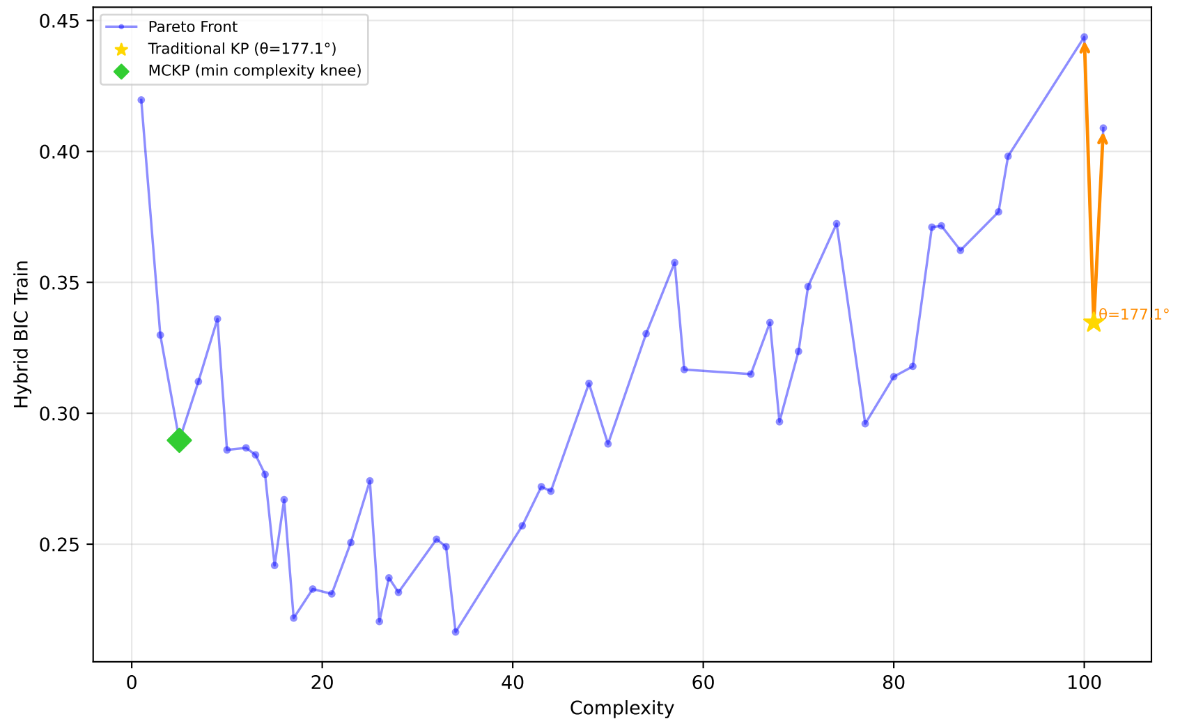
678_visualizing_environmental - Run 17 - SVP - Hybrid BIC Train \lambda_1=0.00, \lambda_2=0.10, \lambda_3=0.20 | Difficulty: 0.26 | Method: mckp
