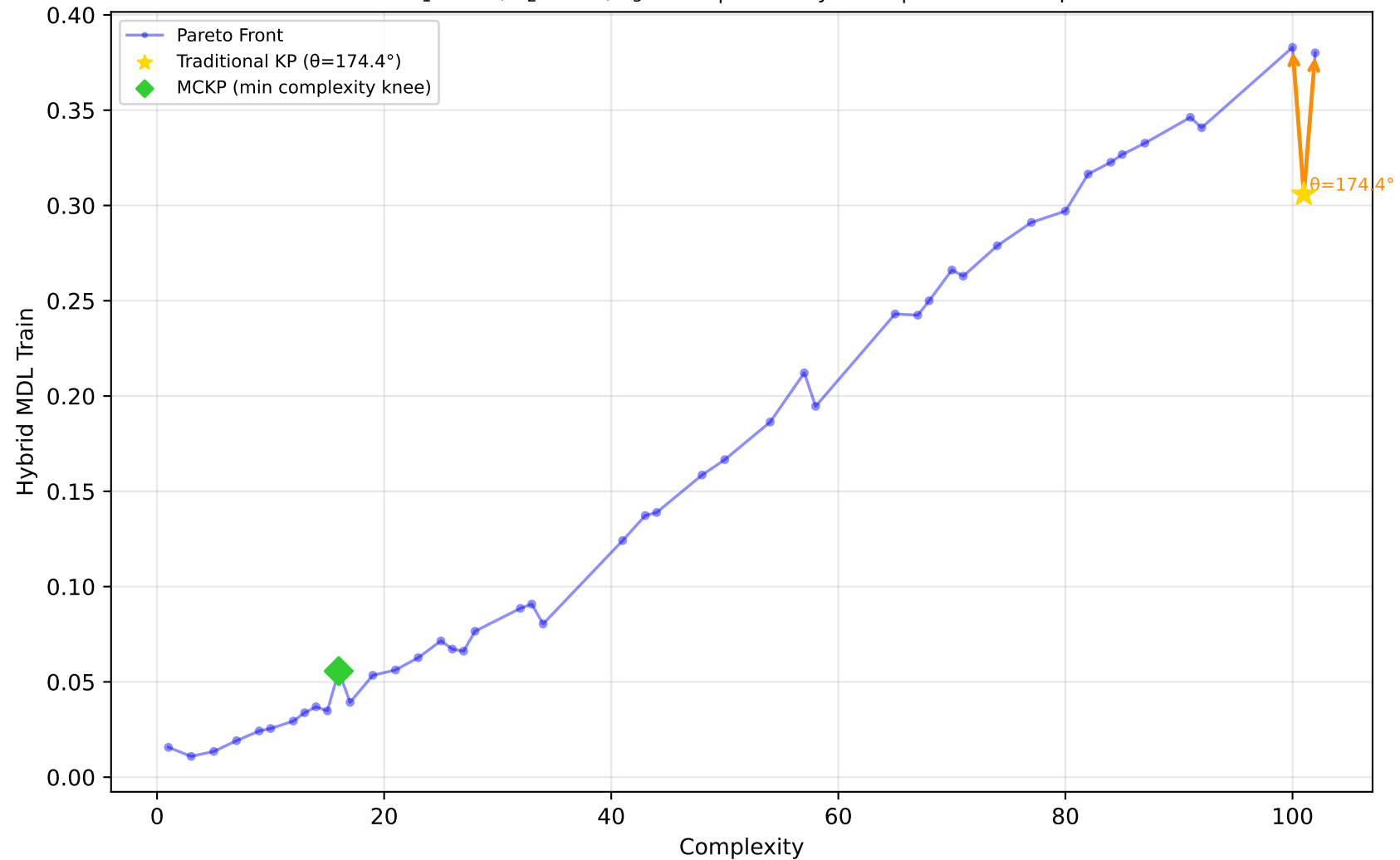
678_visualizing_environmental - Run 17 - SVP - Hybrid MDL Train \lambda_1=0.00, \lambda_2=0.10, \lambda_3=0.20 | Difficulty: 0.26 | Method: mckp
