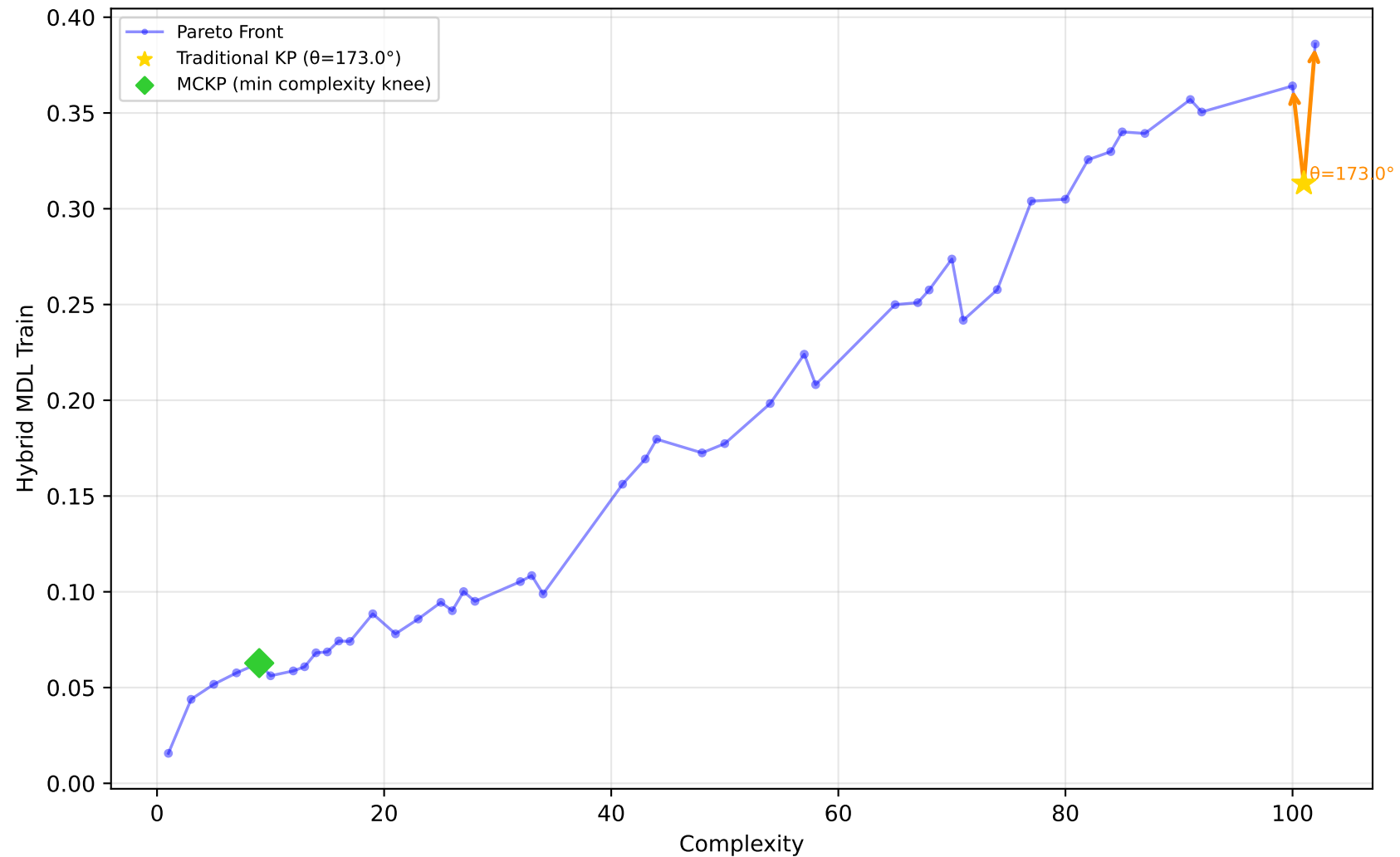
678_visualizing_environmental - Run 17 - SVP - Hybrid MDL Train \lambda_1=0.40 , \lambda_2=0.00 , \lambda_3=0.00 | Difficulty: 0.26 | Method: mckp
