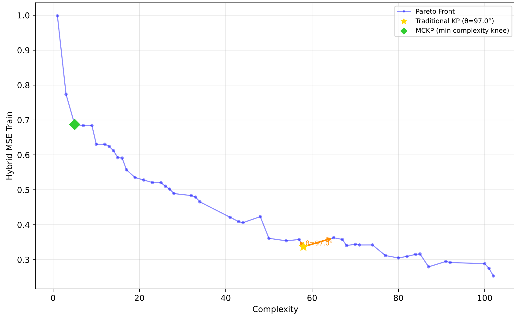
678_visualizing_environmental - Run 17 - SVP - Hybrid MSE Train \lambda_1=0.00, \lambda_2=0.10, \lambda_3=0.20 | Difficulty: 0.26 | Method: mckp
