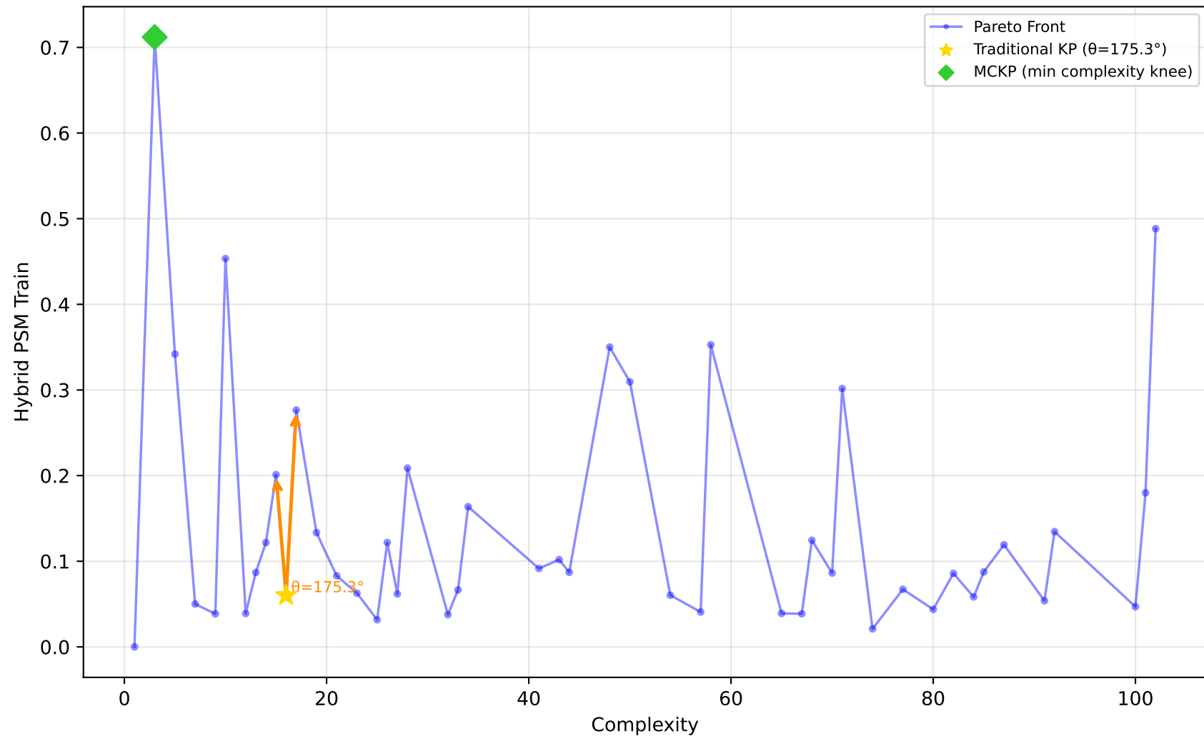
678_visualizing_environmental - Run 17 - SVP - Hybrid PSM Train \lambda_1=0.40, \lambda_2=0.00, \lambda_3=0.00 | Difficulty: 0.26 | Method: mckp
