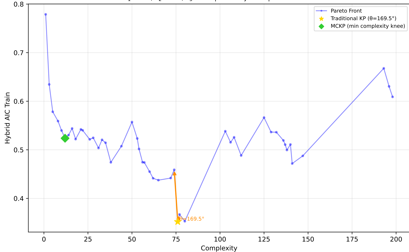
678_visualizing_environmental - Run 18 - MVP - Hybrid AIC Train \lambda_1=0.00, \lambda_2=0.00, \lambda_3=0.10 | Difficulty: 0.73 | Method: hmr
