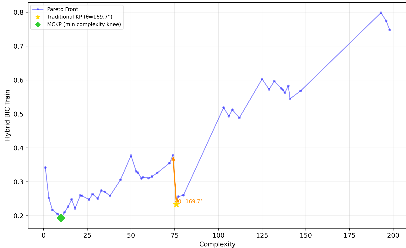
678_visualizing_environmental - Run 18 - MVP - Hybrid BIC Train \lambda_1=0.00, \lambda_2=0.00, \lambda_3=0.10 | Difficulty: 0.73 | Method: hmr
