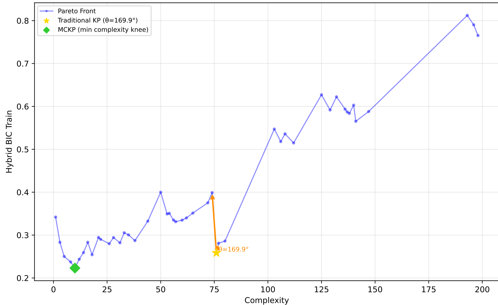
678_visualizing_environmental - Run 18 - MVP - Hybrid BIC Train \lambda_1=0.40, \lambda_2=0.00, \lambda_3=0.00 | Difficulty: 0.73 | Method: hmr
