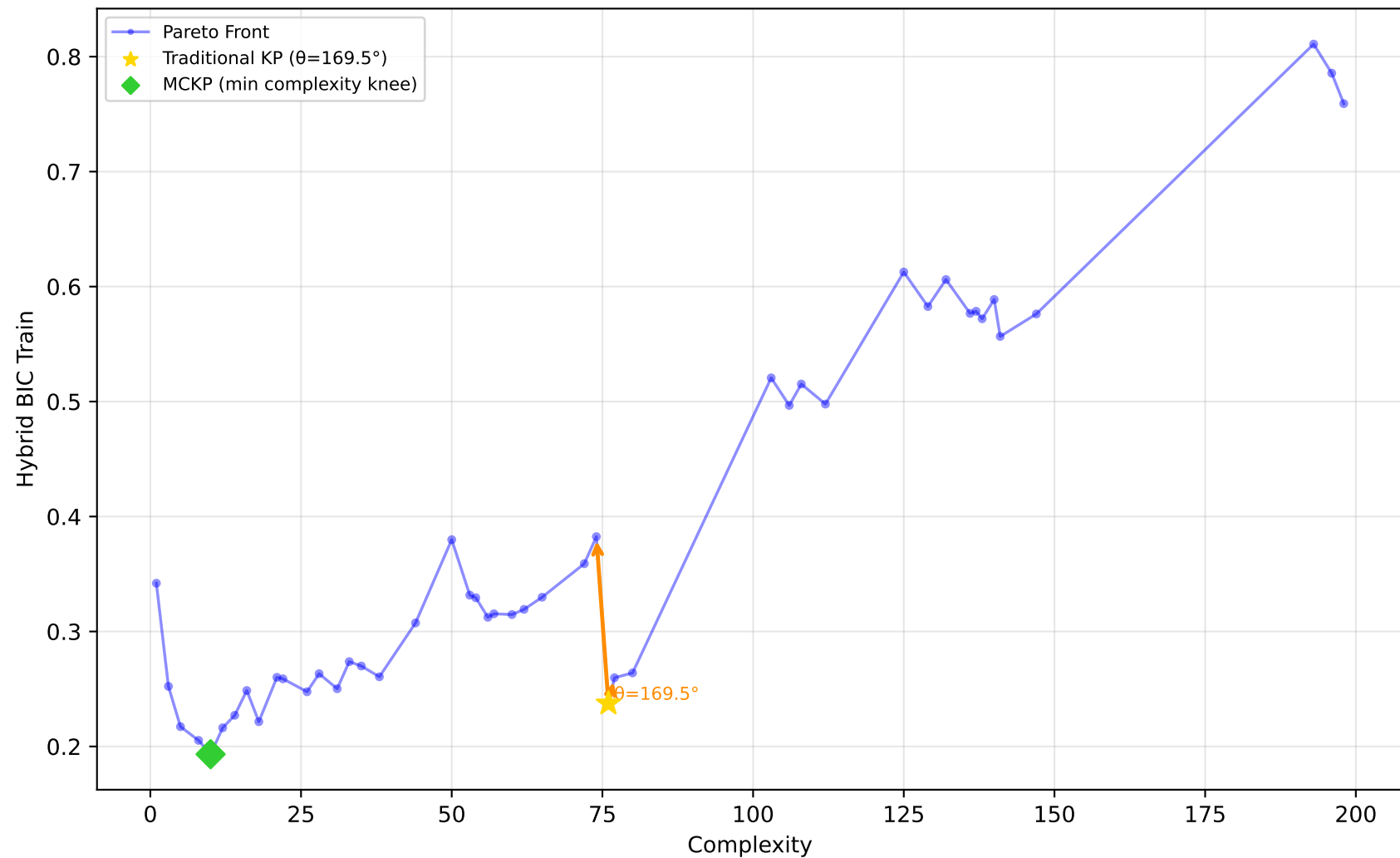
678_visualizing_environmental - Run 18 - SVP - Hybrid BIC Train \lambda_1=0.00, \lambda_2=0.10, \lambda_3=0.20 | Difficulty: 0.73 | Method: hmr
