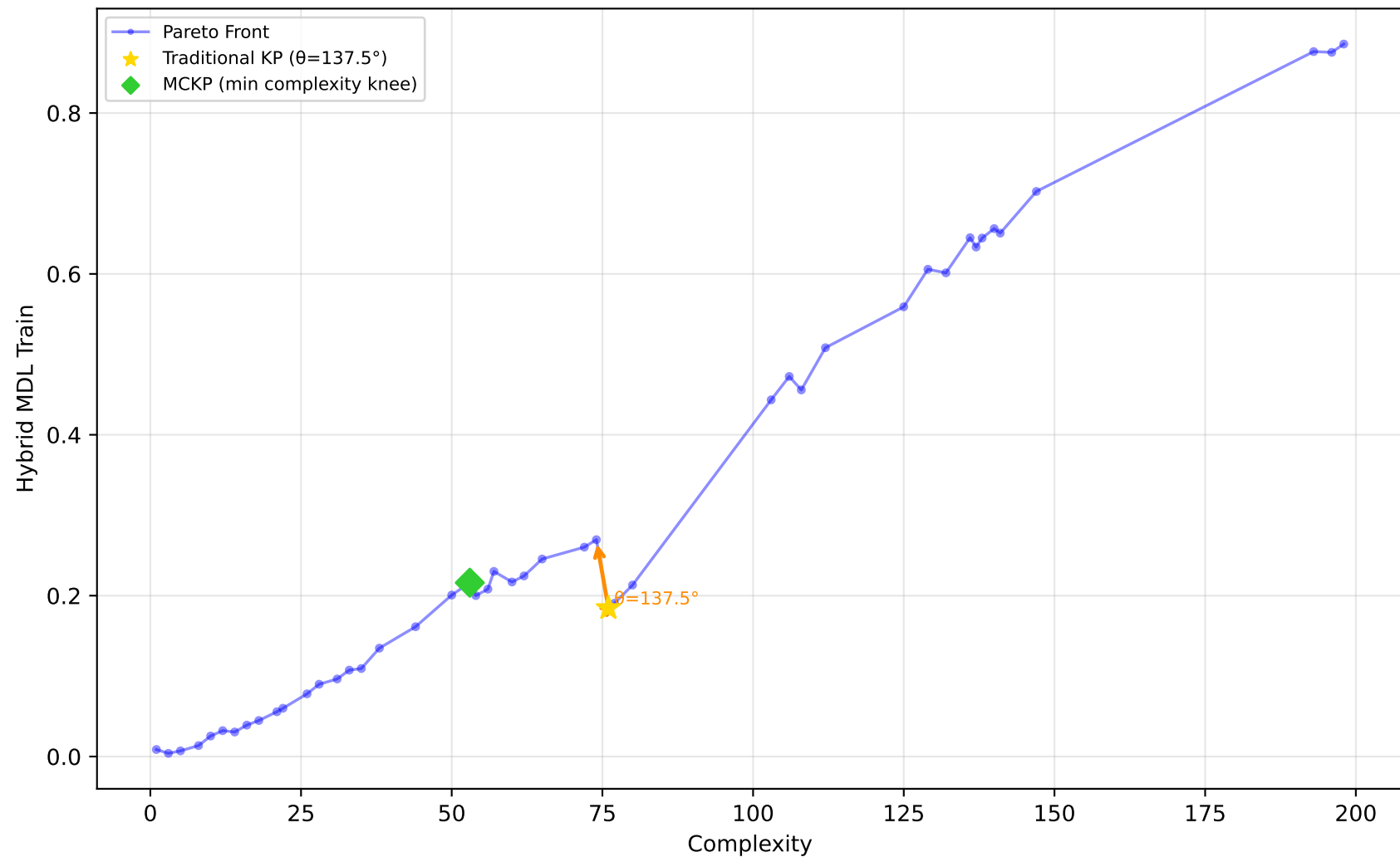
678_visualizing_environmental - Run 18 - SVP - Hybrid MDL Train \lambda_1=0.00, \lambda_2=0.10, \lambda_3=0.20 | Difficulty: 0.73 | Method: hmr
