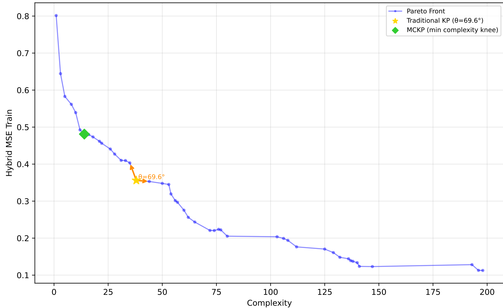
678_visualizing_environmental - Run 18 - SVP - Hybrid MSE Train \lambda_1=0.40, \lambda_2=0.00, \lambda_3=0.00 | Difficulty: 0.73 | Method: hmr
