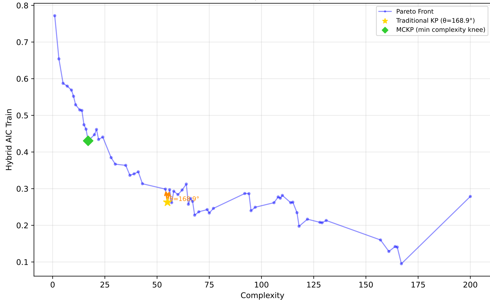
678_visualizing_environmental - Run 19 - MVP - Hybrid AIC Train \lambda_1=0.40, \lambda_2=0.00, \lambda_3=0.00 | Difficulty: 0.20 | Method: mckp
