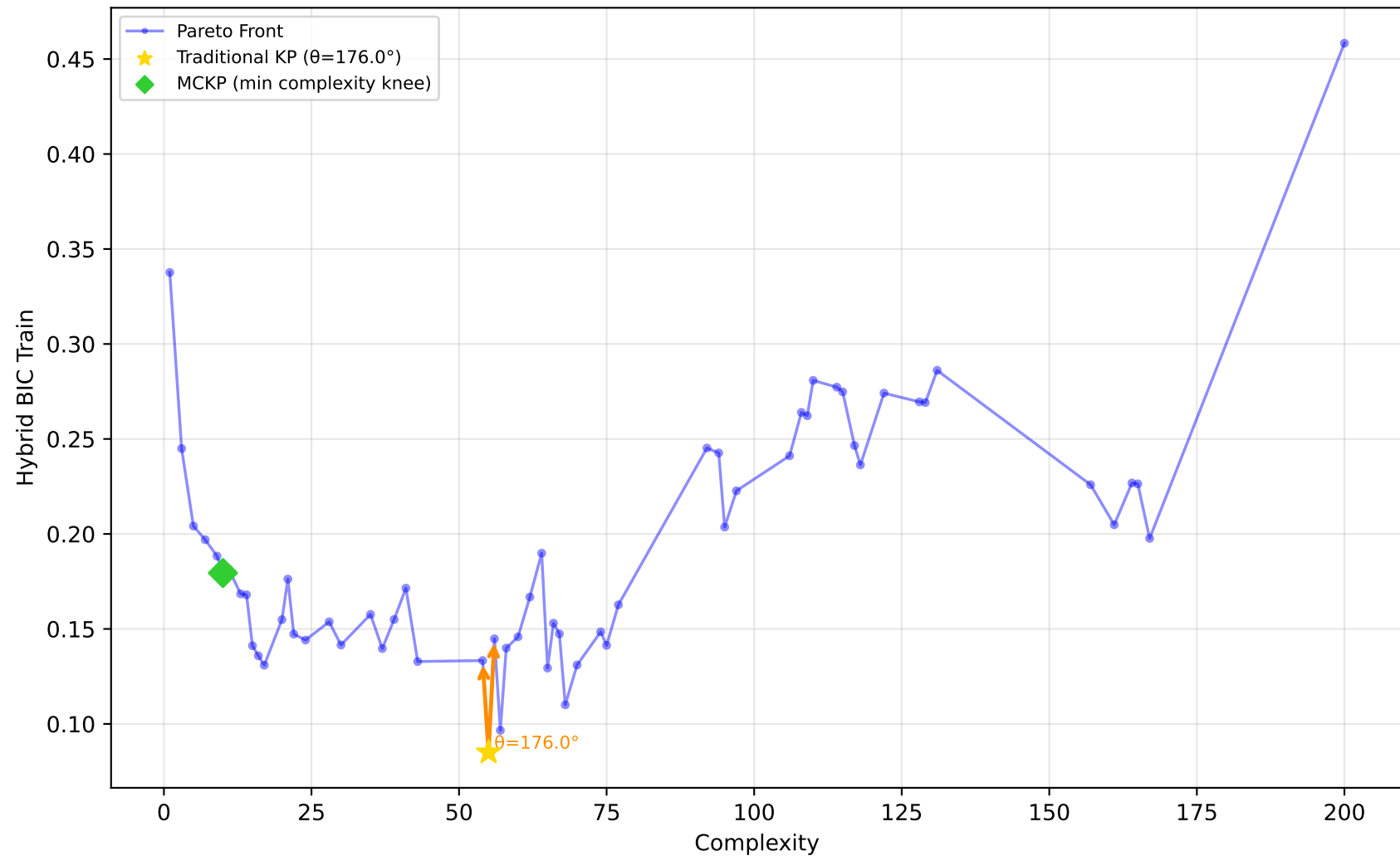
678_visualizing_environmental - Run 19 - MVP - Hybrid BIC Train \lambda_1=0.00, \lambda_2=0.00, \lambda_3=0.10 | Difficulty: 0.20 | Method: mckp
