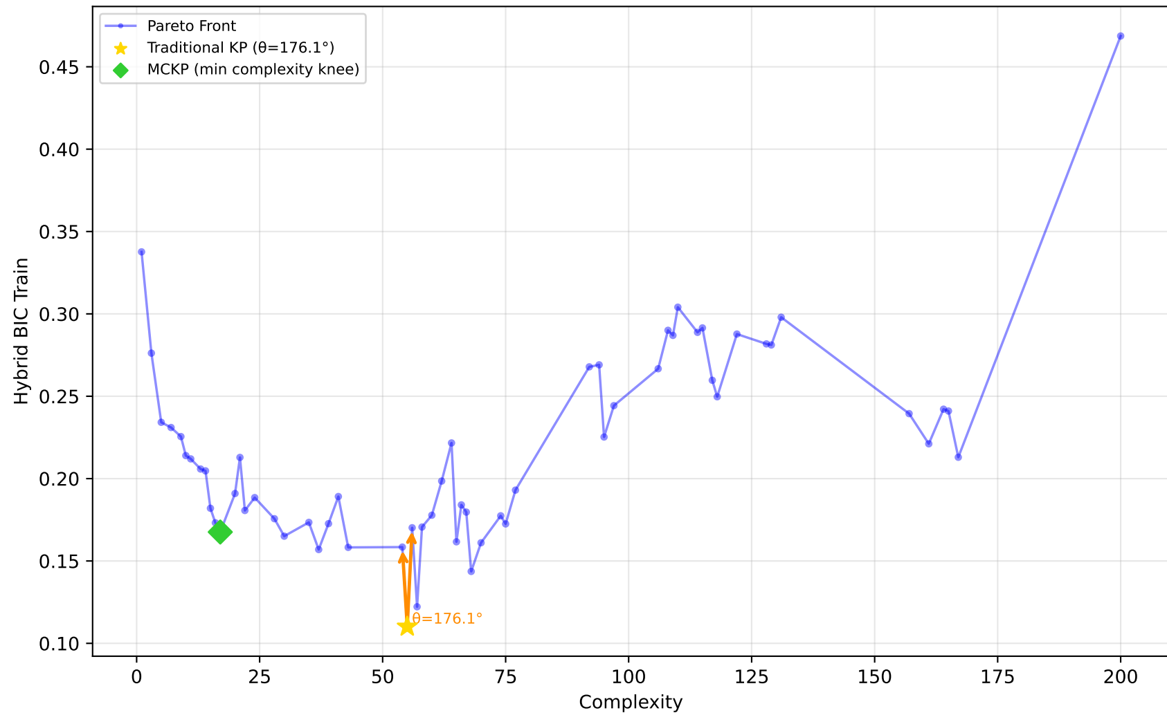
678_visualizing_environmental - Run 19 - MVP - Hybrid BIC Train \lambda_1=0.40, \lambda_2=0.00, \lambda_3=0.00 | Difficulty: 0.20 | Method: mckp
