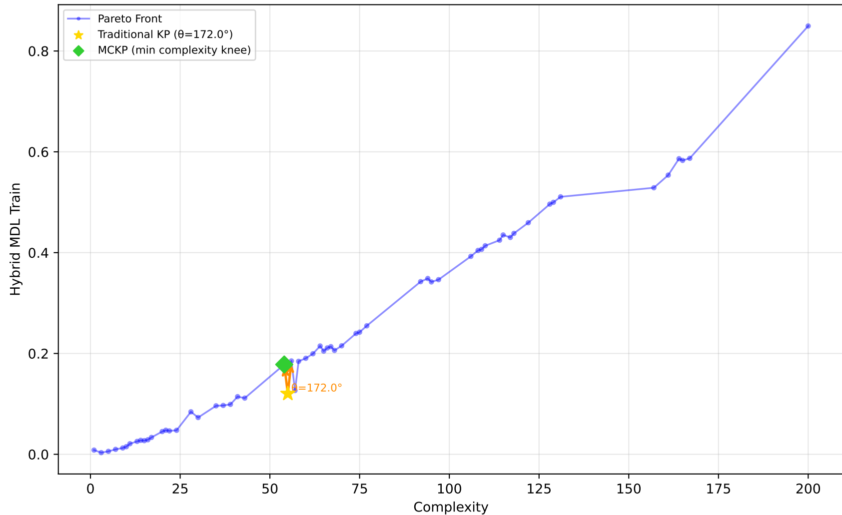
678_visualizing_environmental - Run 19 - MVP - Hybrid MDL Train \lambda_1=0.00, \lambda_2=0.00, \lambda_3=0.10 | Difficulty: 0.20 | Method: mckp
