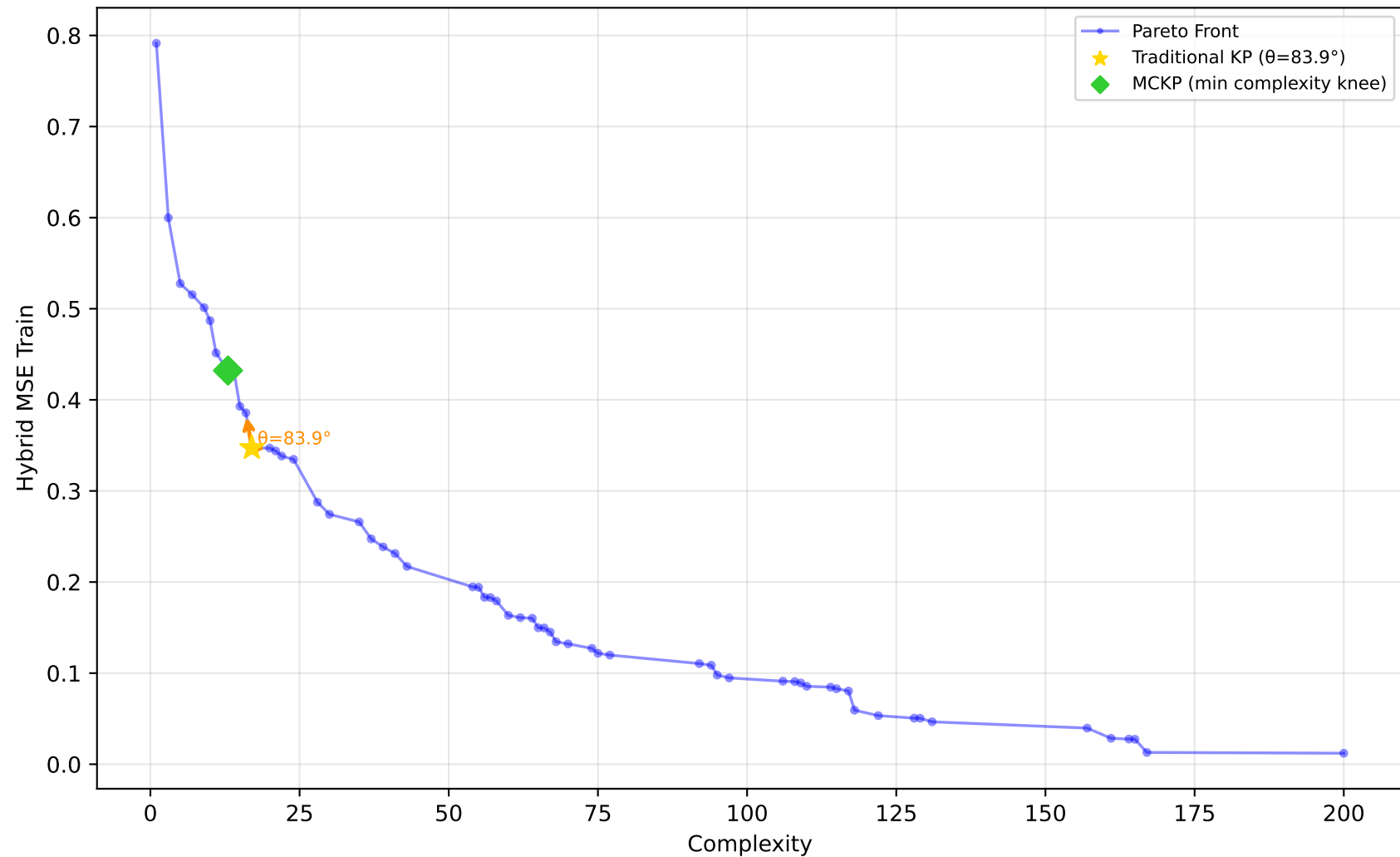
678_visualizing_environmental - Run 19 - MVP - Hybrid MSE Train \lambda_1=0.00, \lambda_2=0.00, \lambda_3=0.10 | Difficulty: 0.20 | Method: mckp
