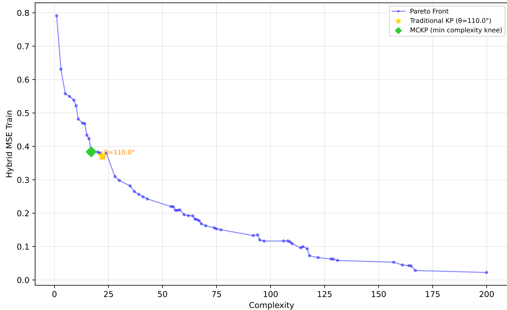
678_visualizing_environmental - Run 19 - MVP - Hybrid MSE Train \lambda_1=0.40, \lambda_2=0.00, \lambda_3=0.00 | Difficulty: 0.20 | Method: mckp
