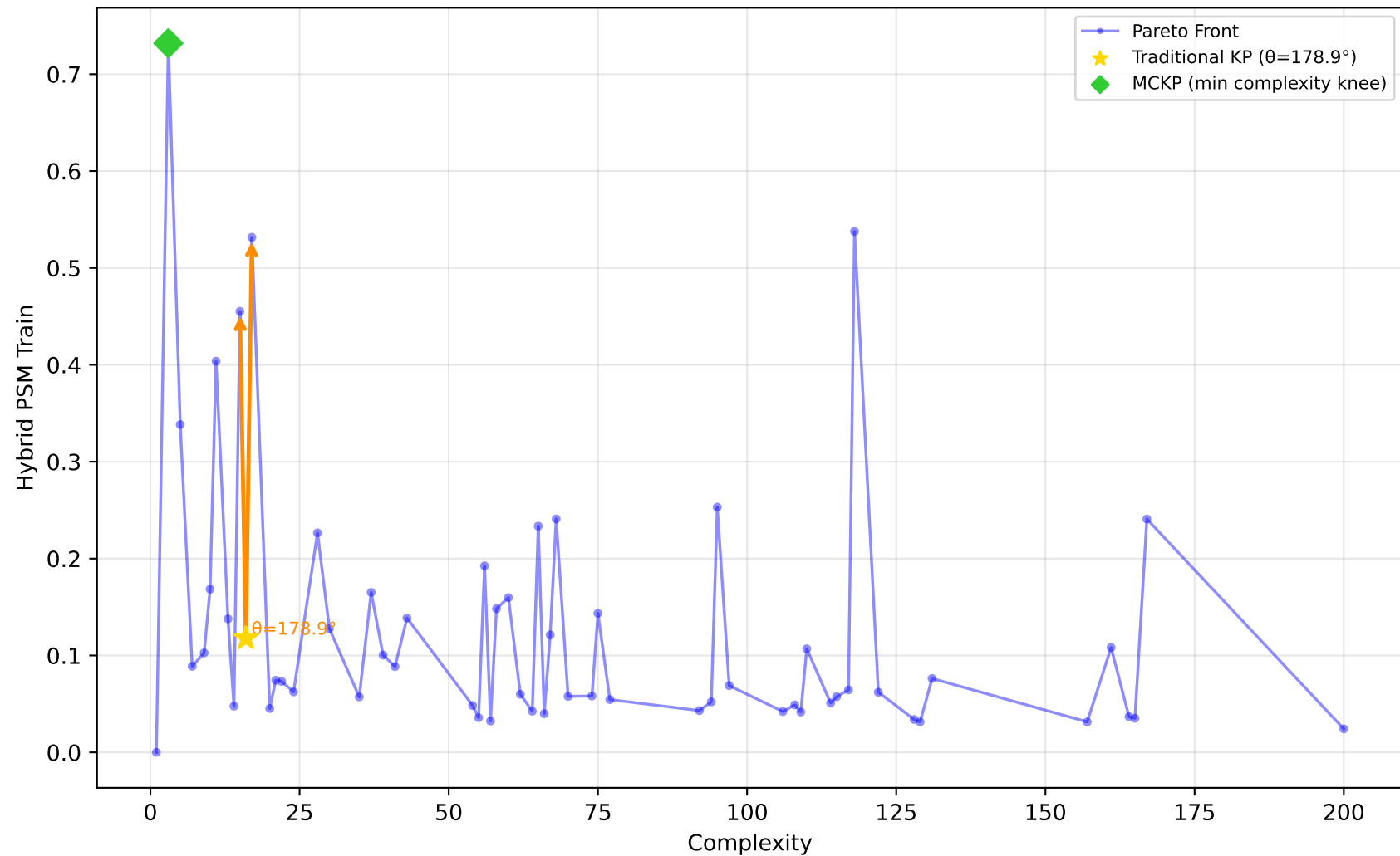
678_visualizing_environmental - Run 19 - MVP - Hybrid PSM Train \lambda_1=0.40, \lambda_2=0.00, \lambda_3=0.00 | Difficulty: 0.20 | Method: mckp
