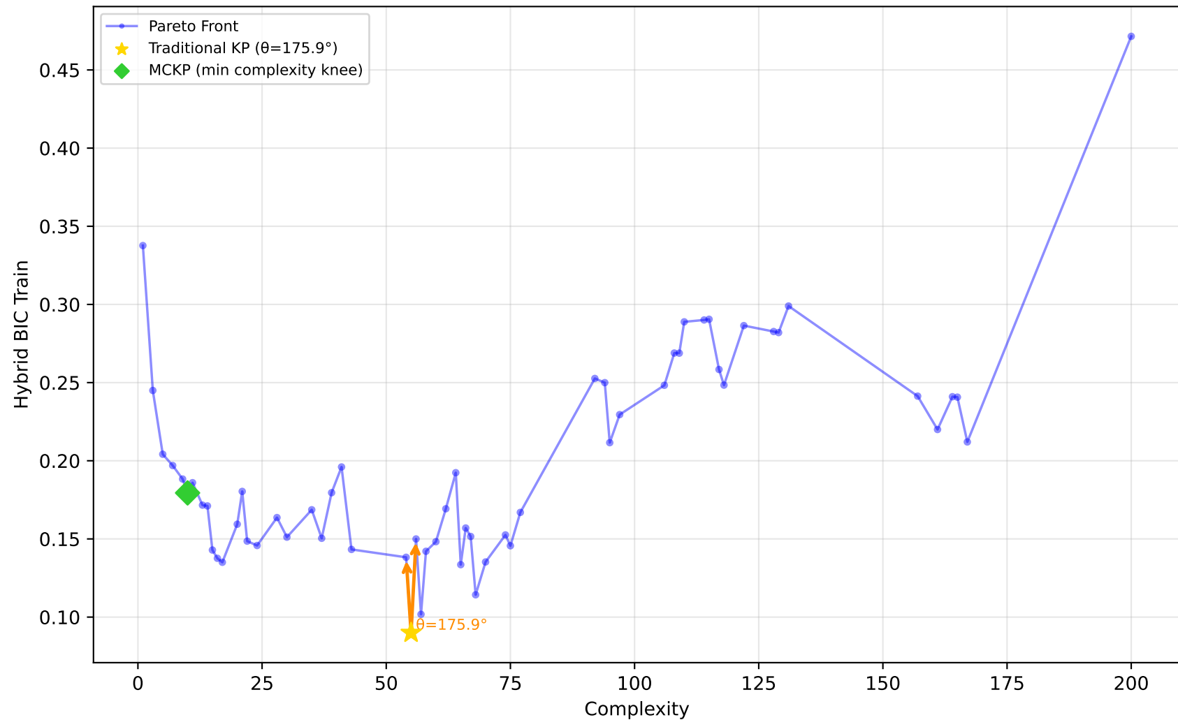
678_visualizing_environmental - Run 19 - SVP - Hybrid BIC Train \lambda_1=0.00, \lambda_2=0.10, \lambda_3=0.20 | Difficulty: 0.20 | Method: mckp
