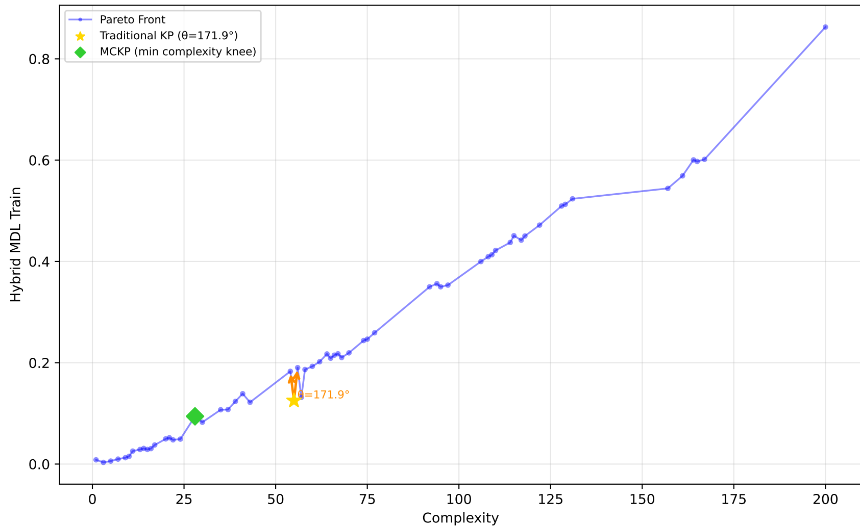
678_visualizing_environmental - Run 19 - SVP - Hybrid MDL Train \lambda_1=0.00, \lambda_2=0.10, \lambda_3=0.20 | Difficulty: 0.20 | Method: mckp
