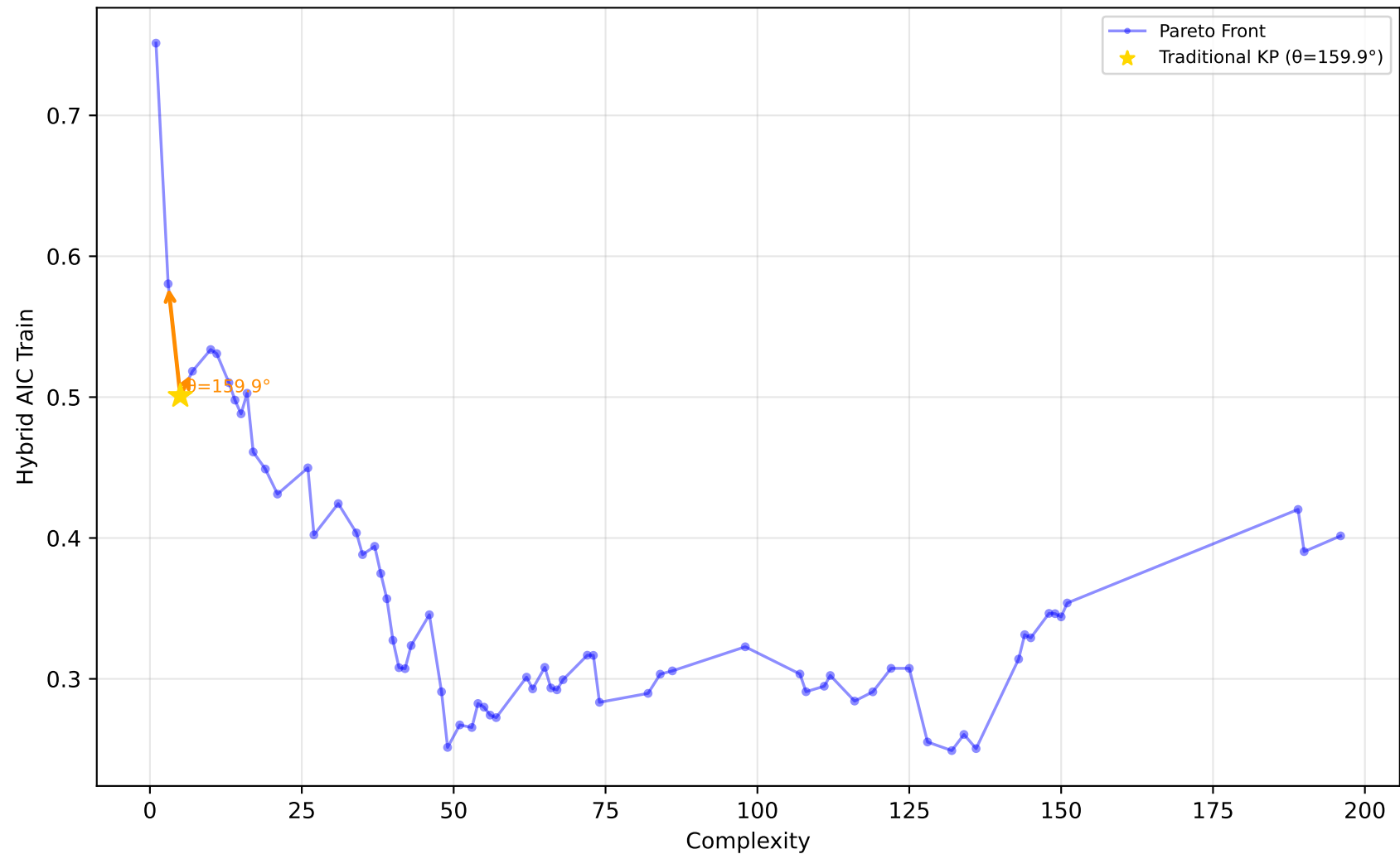
678_visualizing_environmental - Run 1 - MVP - Hybrid AIC Train \lambda_1=0.00, \lambda_2=0.00, \lambda_3=0.10 | Difficulty: 0.35 | Method: mckp
