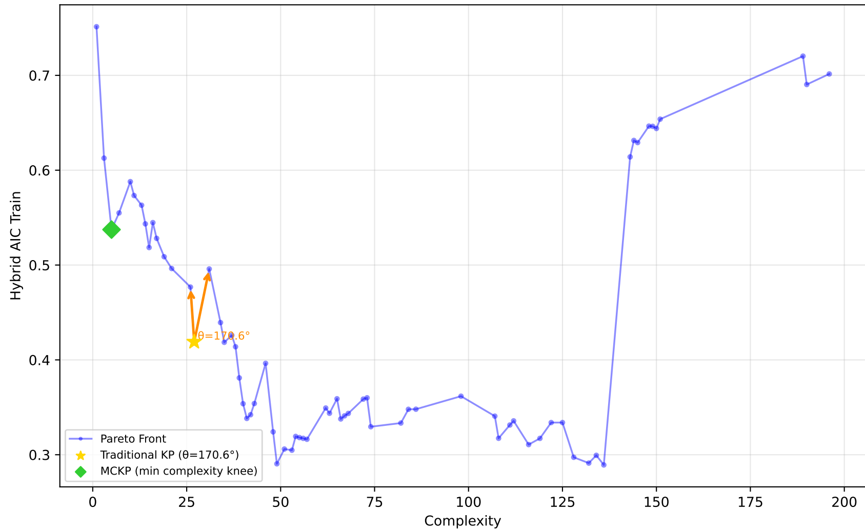
678_visualizing_environmental - Run 1 - MVP - Hybrid AIC Train \lambda_1=0.40 , \lambda_2=0.00 , \lambda_3=0.00 | Difficulty: 0.35 | Method: mckp
