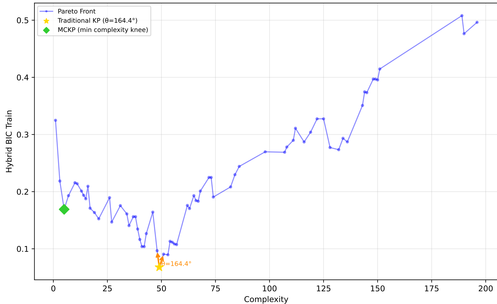
678_visualizing_environmental - Run 1 - MVP - Hybrid BIC Train \lambda_1=0.00, \lambda_2=0.00, \lambda_3=0.10 | Difficulty: 0.35 | Method: mckp
