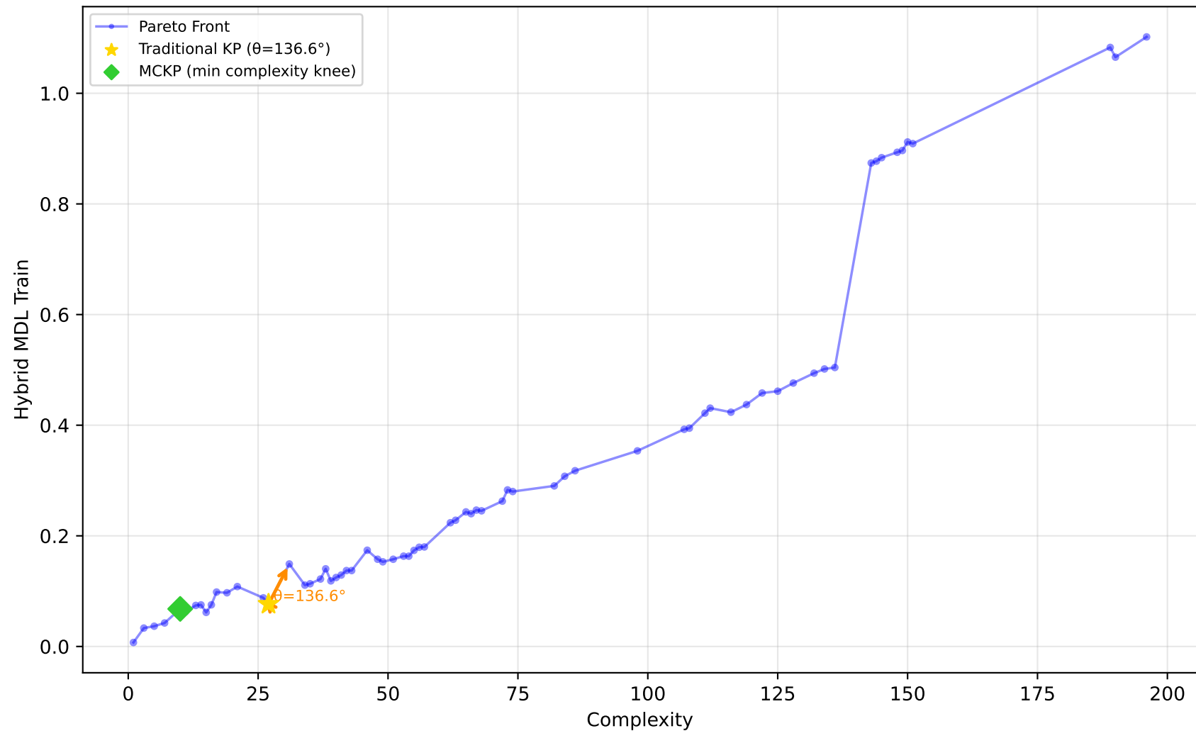
678_visualizing_environmental - Run 1 - MVP - Hybrid MDL Train \lambda_1=0.40 , \lambda_2=0.00 , \lambda_3=0.00 | Difficulty: 0.35 | Method: mckp
