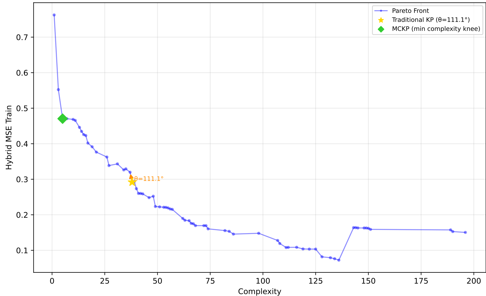
678_visualizing_environmental - Run 1 - MVP - Hybrid MSE Train \lambda_1=0.00, \lambda_2=0.00, \lambda_3=0.10 | Difficulty: 0.35 | Method: mckp
