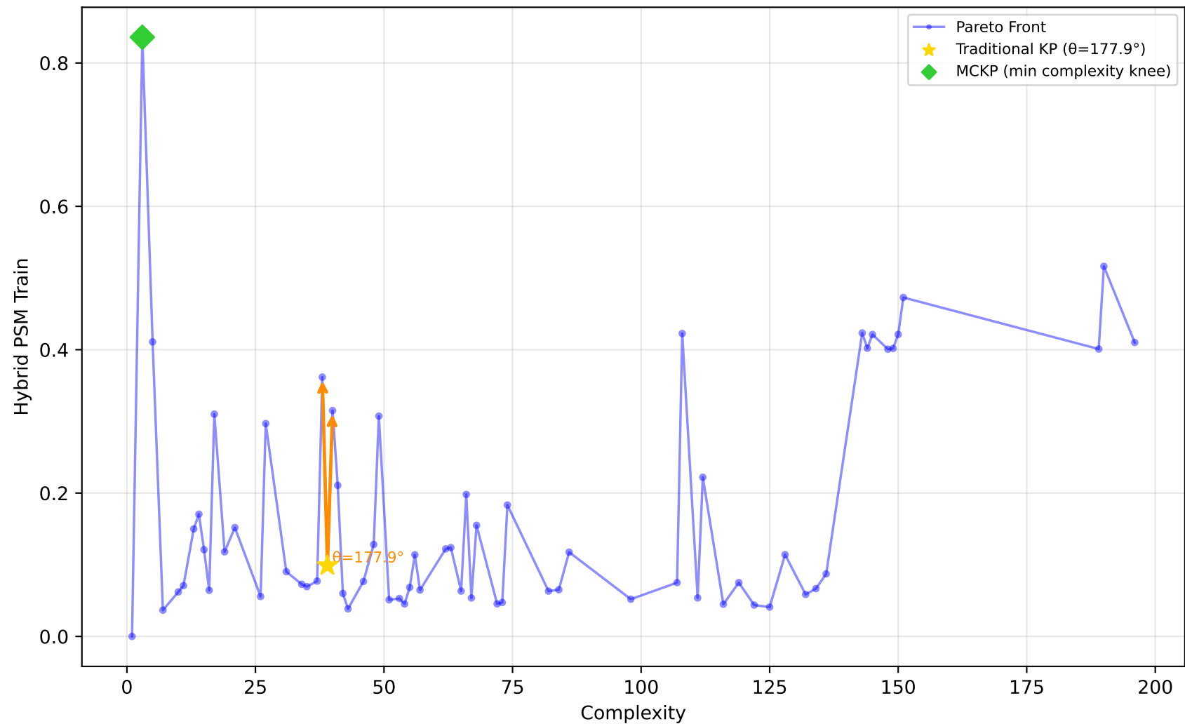
678_visualizing_environmental - Run 1 - MVP - Hybrid PSM Train \lambda_1=0.40, \lambda_2=0.00, \lambda_3=0.00 | Difficulty: 0.35 | Method: mckp
