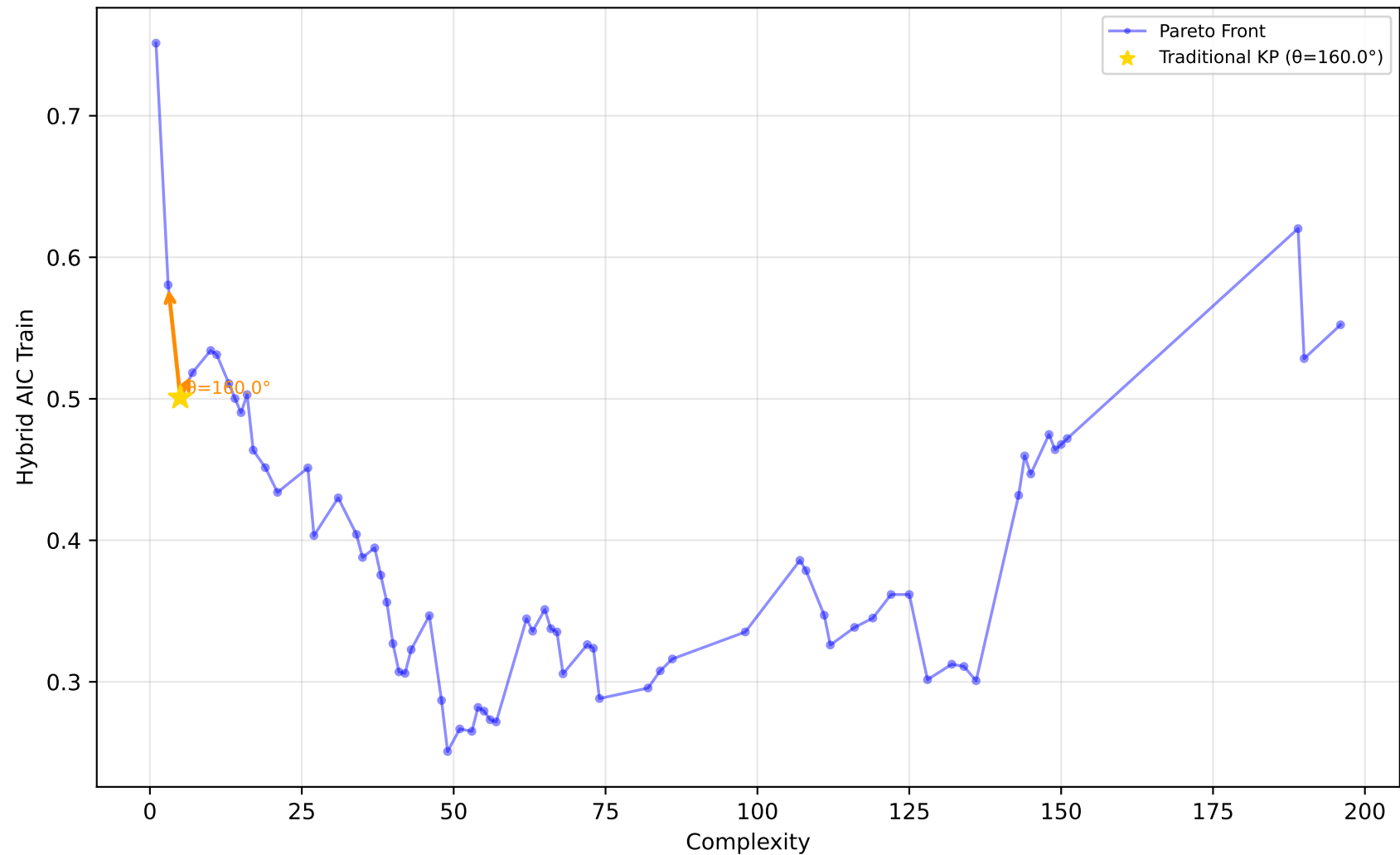
678_visualizing_environmental - Run 1 - SVP - Hybrid AIC Train \lambda_1=0.00, \lambda_2=0.10, \lambda_3=0.20 | Difficulty: 0.35 | Method: mckp
