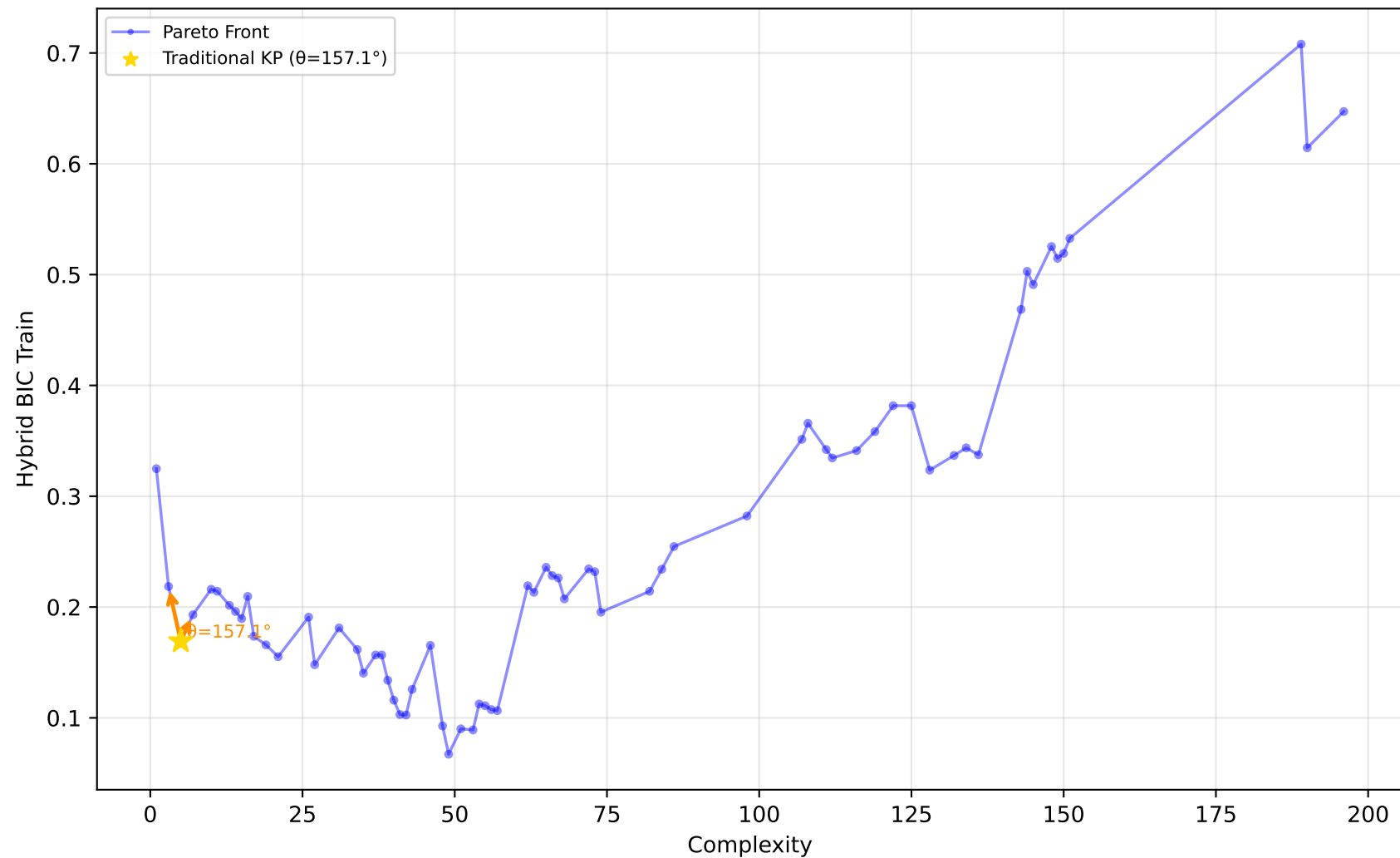
678_visualizing_environmental - Run 1 - SVP - Hybrid BIC Train \lambda_1=0.00, \lambda_2=0.10, \lambda_3=0.20 | Difficulty: 0.35 | Method: mckp
