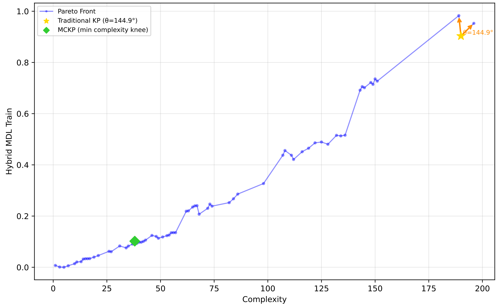
678_visualizing_environmental - Run 1 - SVP - Hybrid MDL Train \lambda_1=0.00, \lambda_2=0.10, \lambda_3=0.20 | Difficulty: 0.35 | Method: mckp
