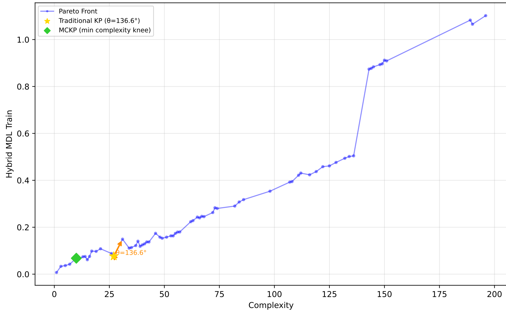
678_visualizing_environmental - Run 1 - SVP - Hybrid MDL Train \lambda_1=0.40, \lambda_2=0.00, \lambda_3=0.00 | Difficulty: 0.35 | Method: mckp
