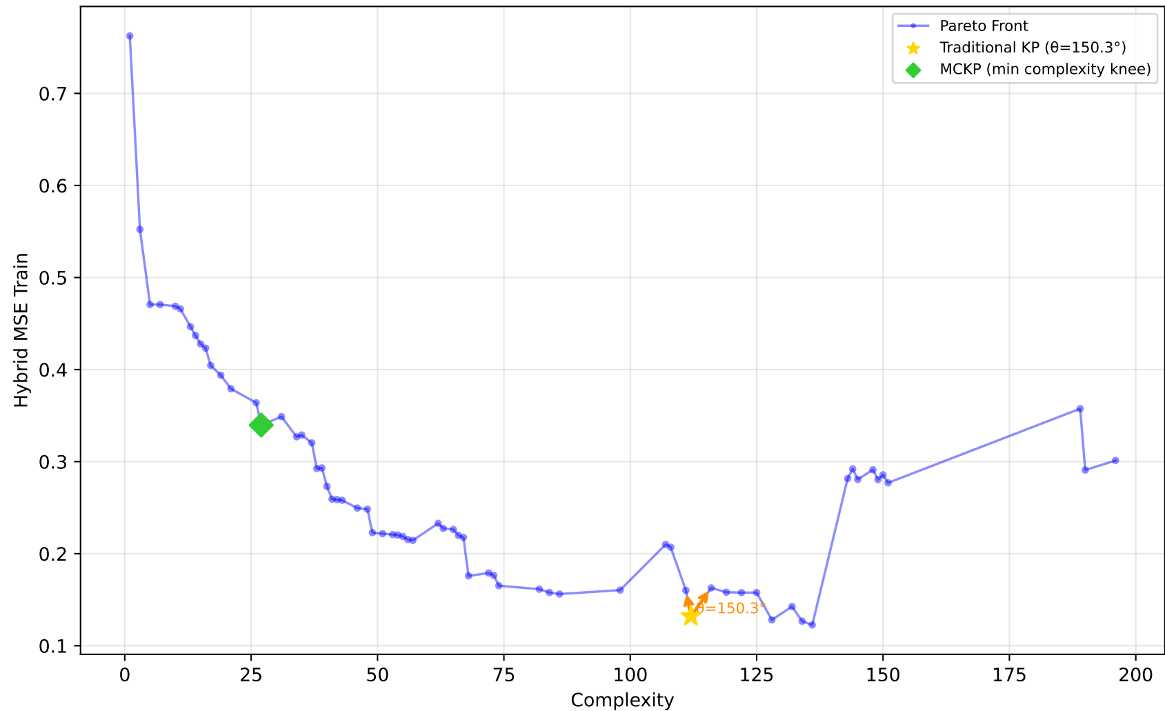
678_visualizing_environmental - Run 1 - SVP - Hybrid MSE Train \lambda_1=0.00, \lambda_2=0.10, \lambda_3=0.20 | Difficulty: 0.35 | Method: mckp
