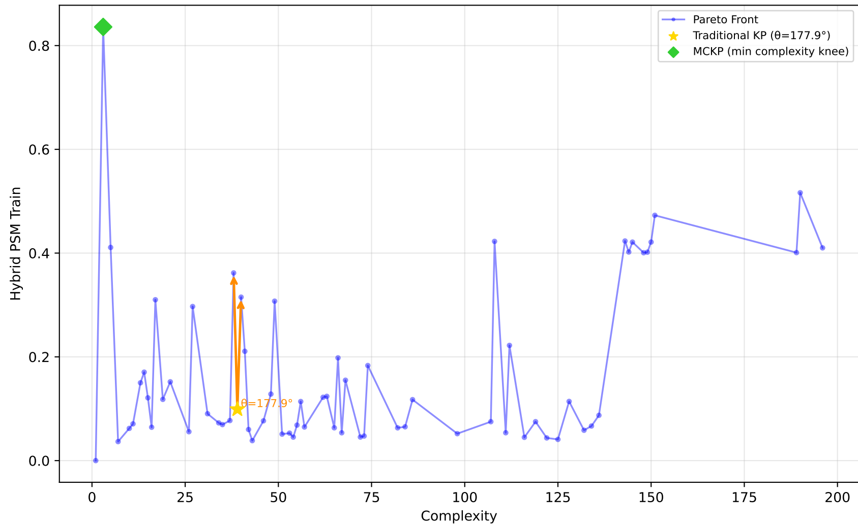
678_visualizing_environmental - Run 1 - SVP - Hybrid PSM Train \lambda_1=0.40 , \lambda_2=0.00 , \lambda_3=0.00 | Difficulty: 0.35 | Method: mckp
