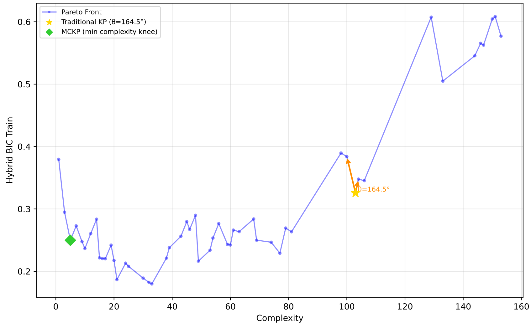
678_visualizing_environmental - Run 20 - MVP - Hybrid BIC Train \lambda_1=0.40, \lambda_2=0.00, \lambda_3=0.00 | Difficulty: 0.75 | Method: hmr
