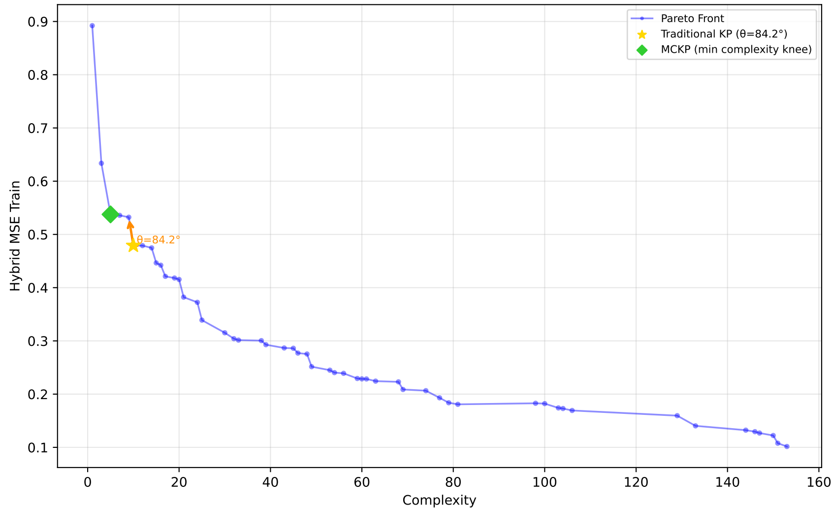
678_visualizing_environmental - Run 20 - MVP - Hybrid MSE Train \lambda_1=0.00, \lambda_2=0.00, \lambda_3=0.10 | Difficulty: 0.75 | Method: hmr
