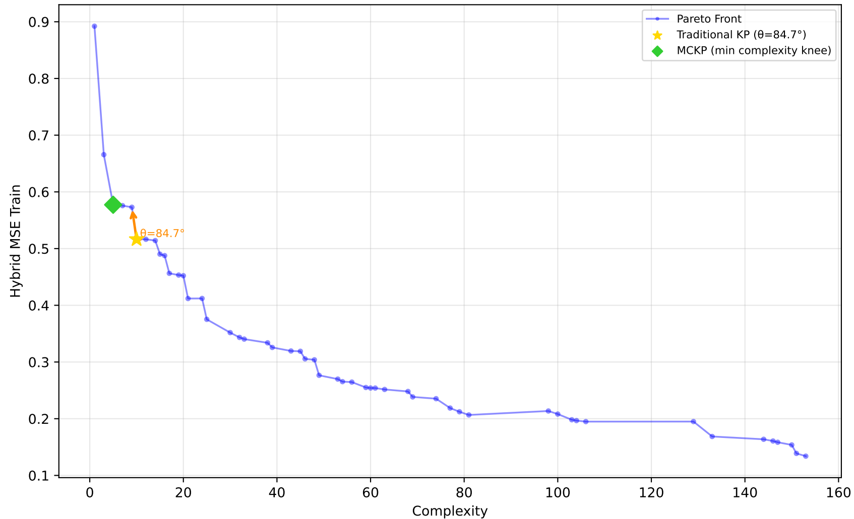
678_visualizing_environmental - Run 20 - MVP - Hybrid MSE Train \lambda_1=0.40, \lambda_2=0.00, \lambda_3=0.00 | Difficulty: 0.75 | Method: hmr
