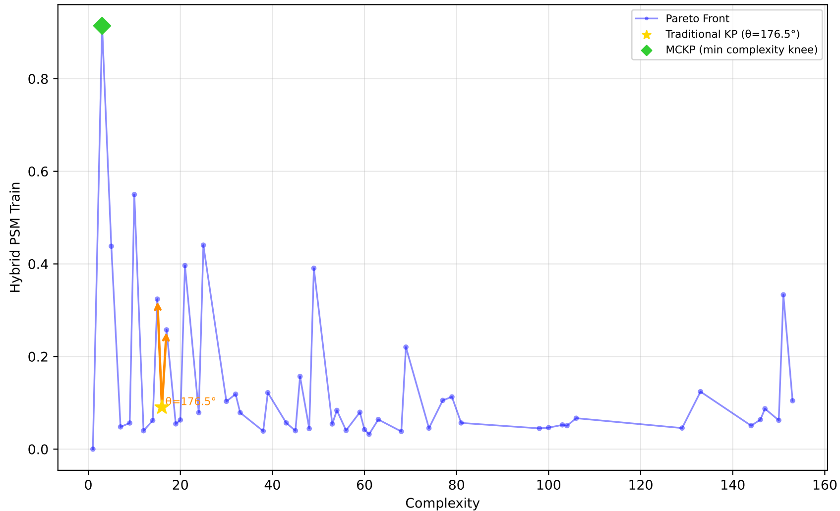
678_visualizing_environmental - Run 20 - MVP - Hybrid PSM Train \lambda_1=0.40, \lambda_2=0.00, \lambda_3=0.00 | Difficulty: 0.75 | Method: hmr
