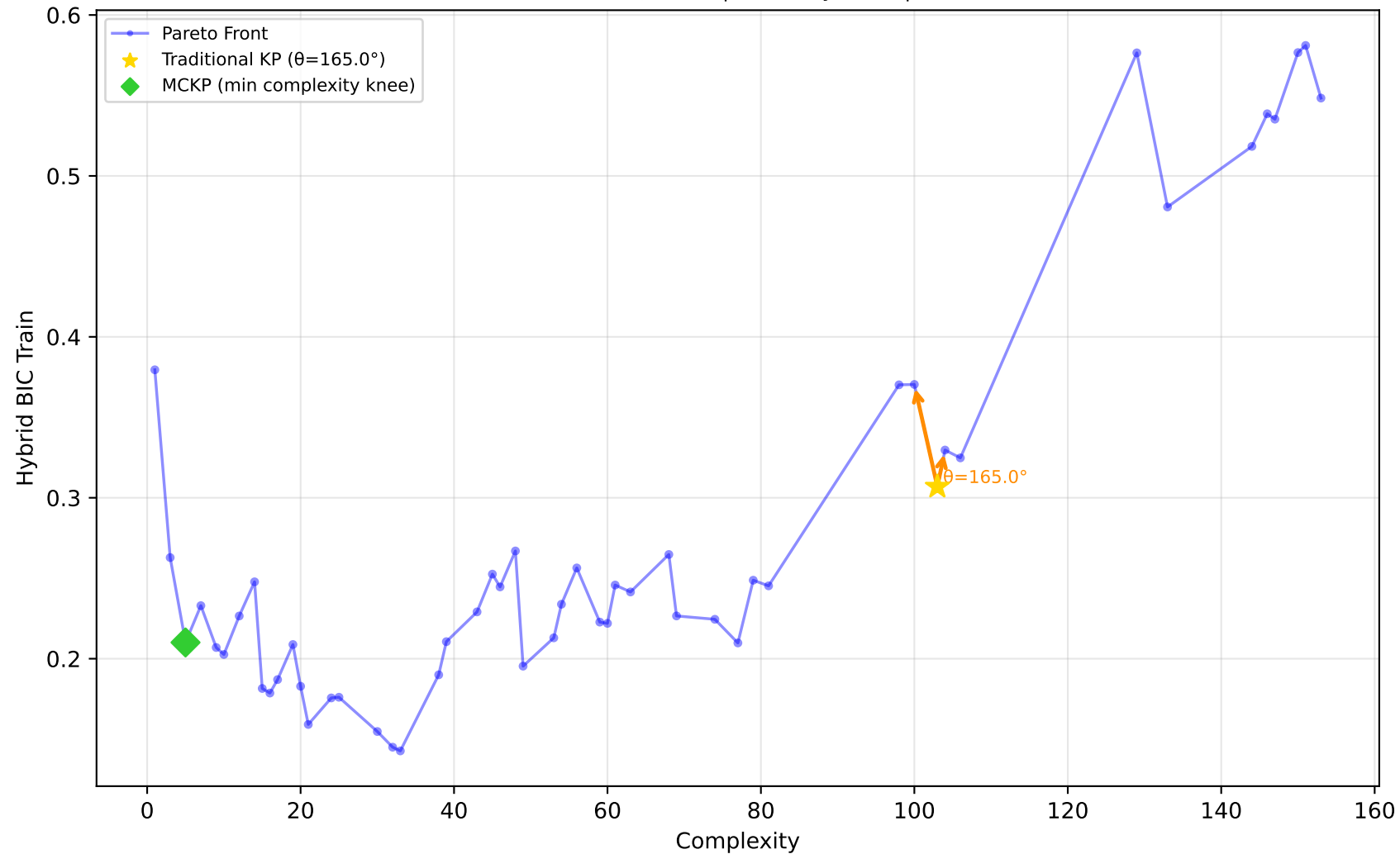
678_visualizing_environmental - Run 20 - SVP - Hybrid BIC Train \lambda_1=0.00, \lambda_2=0.10, \lambda_3=0.20 | Difficulty: 0.75 | Method: hmr
