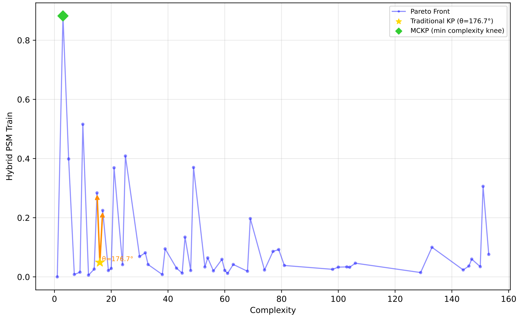
678_visualizing_environmental - Run 20 - SVP - Hybrid PSM Train \lambda_1=0.00, \lambda_2=0.10, \lambda_3=0.20 | Difficulty: 0.75 | Method: hmr
