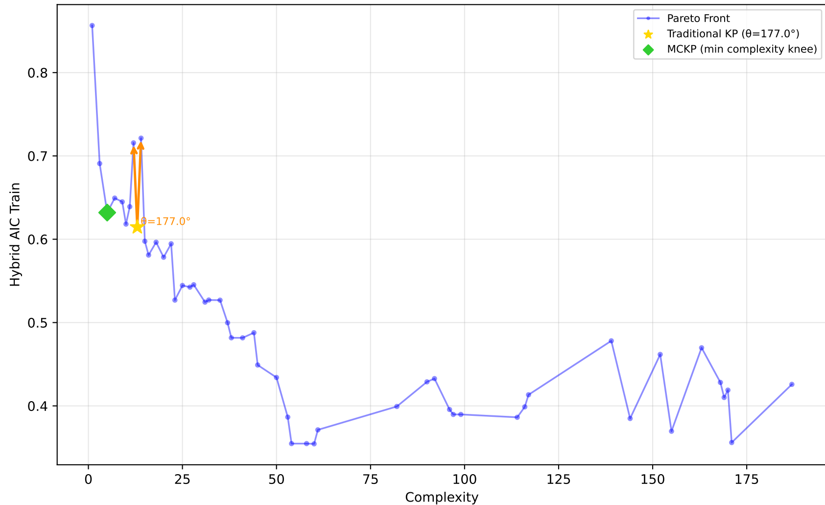
678_visualizing_environmental - Run 21 - MVP - Hybrid AIC Train \lambda_1=0.00, \lambda_2=0.00, \lambda_3=0.10 | Difficulty: 0.09 | Method: mckp
