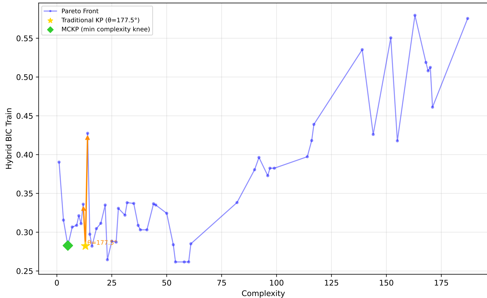
678_visualizing_environmental - Run 21 - MVP - Hybrid BIC Train \lambda_1=0.40, \lambda_2=0.00, \lambda_3=0.00 | Difficulty: 0.09 | Method: mckp
