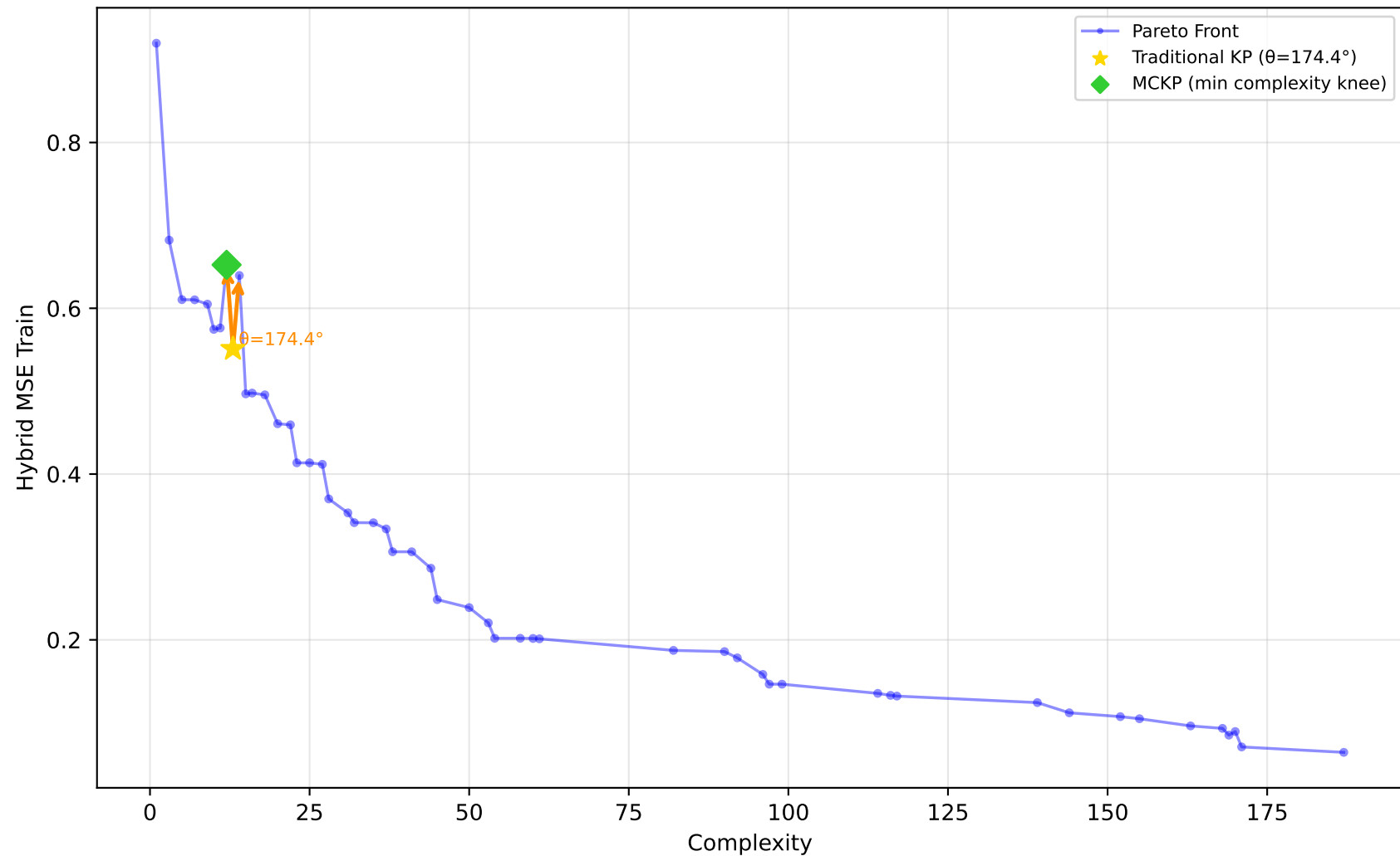
678_visualizing_environmental - Run 21 - MVP - Hybrid MSE Train \lambda_1=0.00, \lambda_2=0.00, \lambda_3=0.10 | Difficulty: 0.09 | Method: mckp
